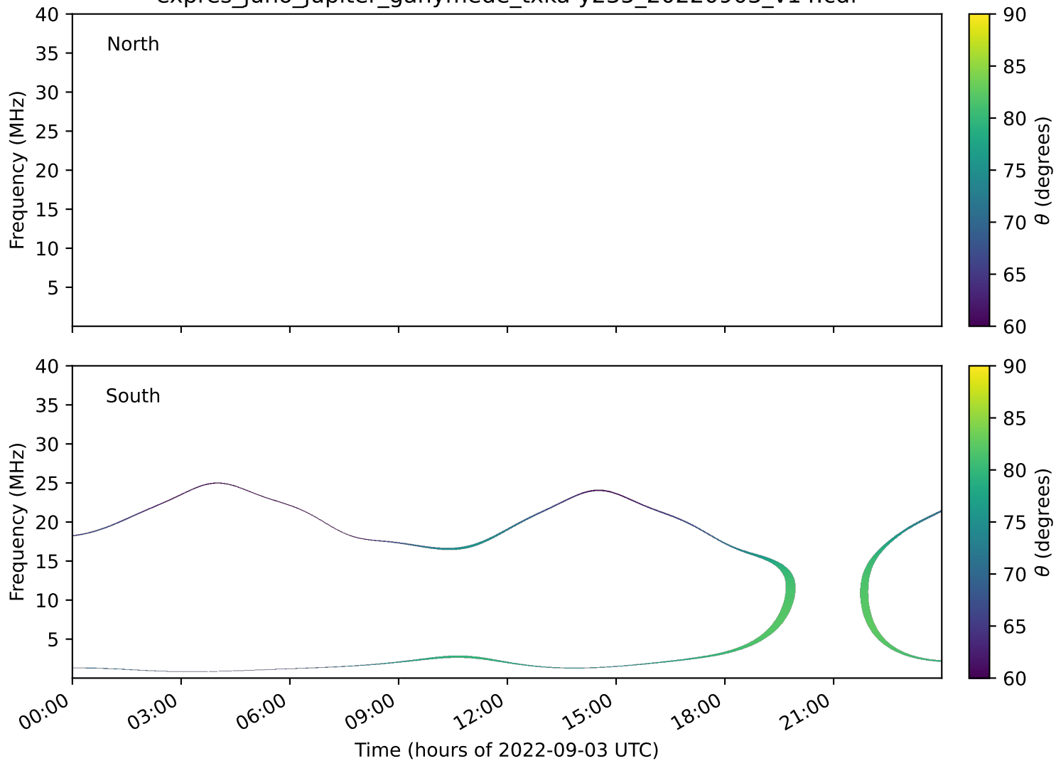
expres_juno_jupiter_ganymede_txka-y235_20220903_v14.cdf
