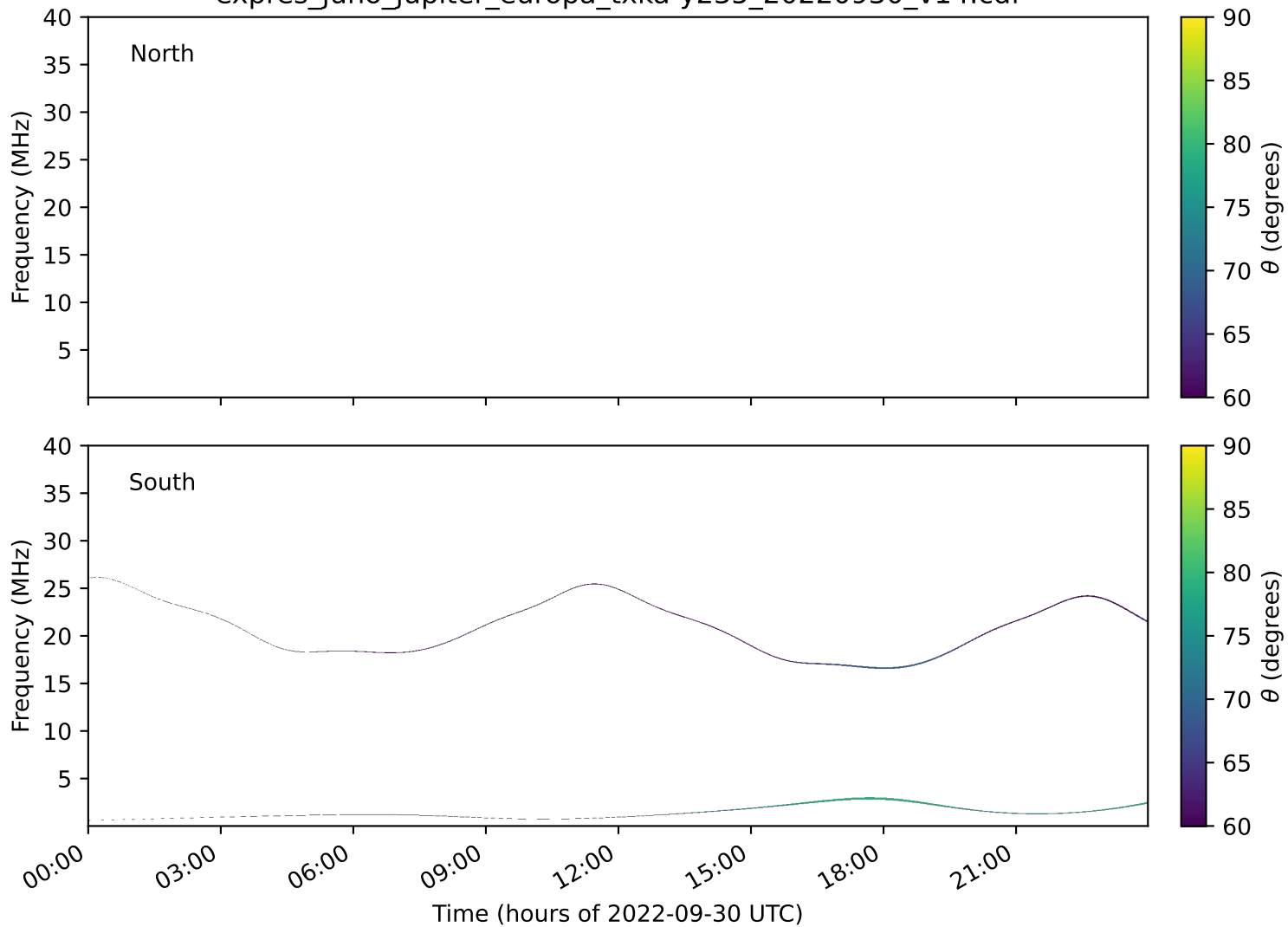
expres_juno_jupiter_europa_txka-y235_20220930_v14.cdf
