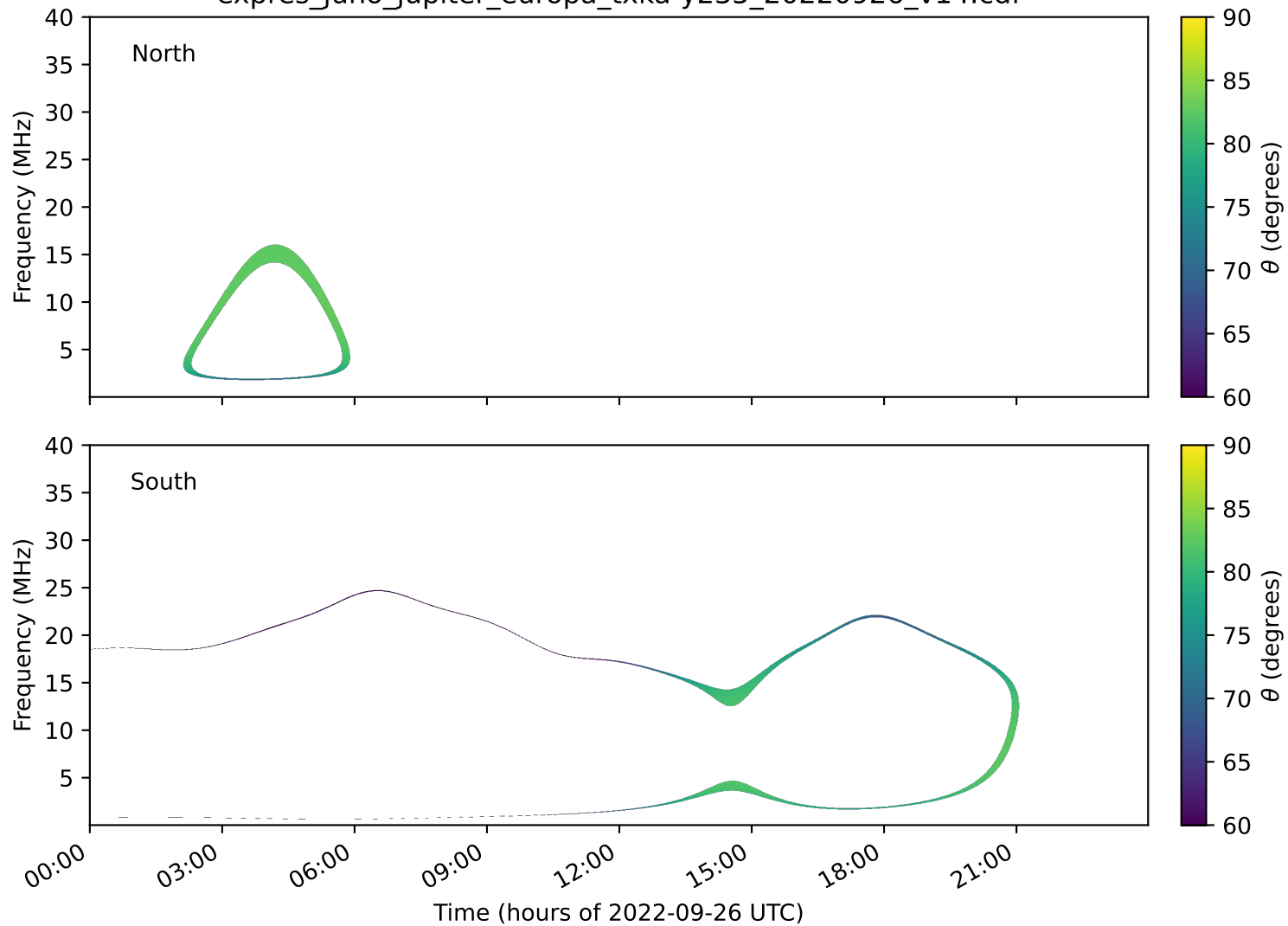
expres_juno_jupiter_europa_txka-y235_20220926_v14.cdf
