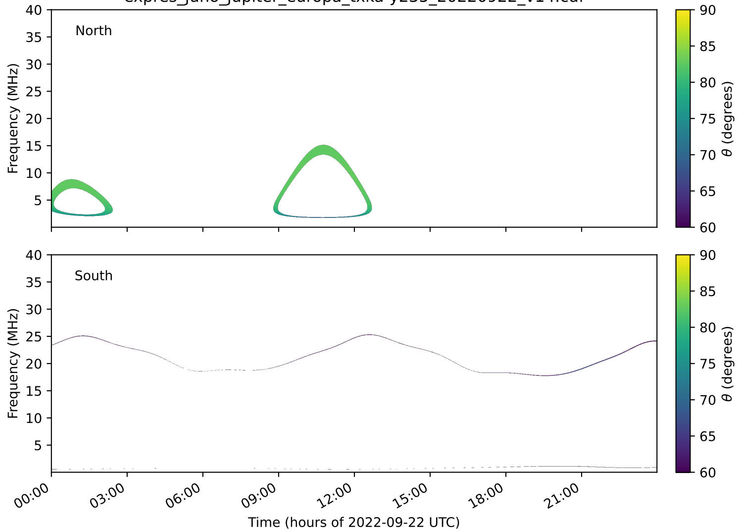
expres_juno_jupiter_europa_txka-y235_20220922_v14.cdf
