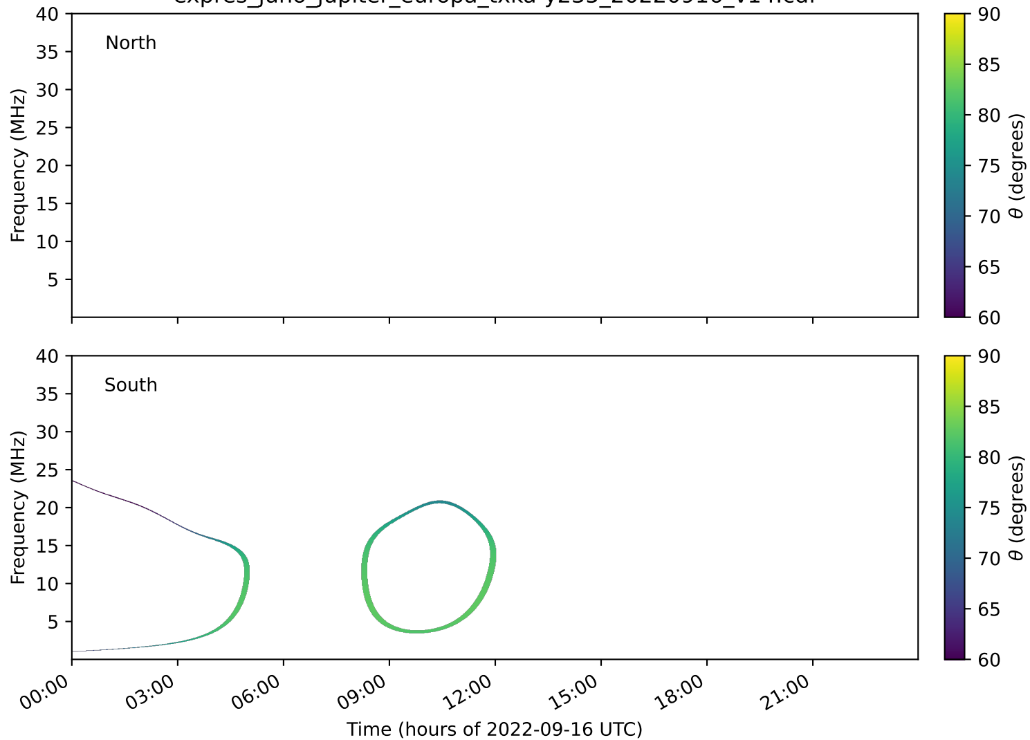
expres_juno_jupiter_europa_txka-y235_20220916_v14.cdf
