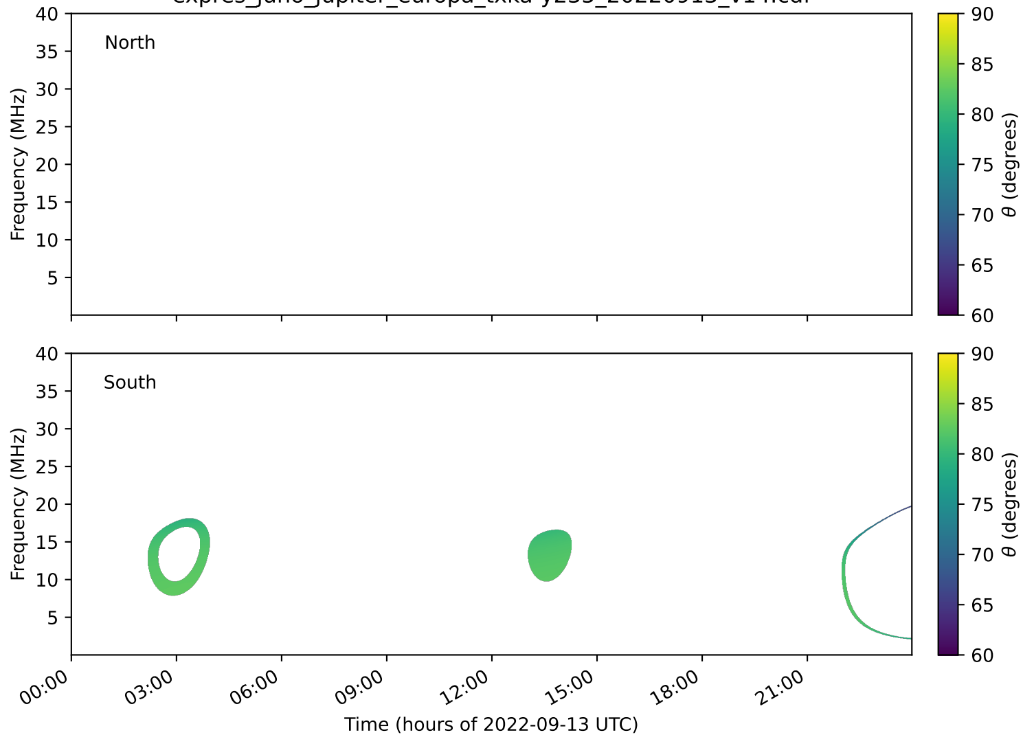
expres_juno_jupiter_europa_txka-y235_20220913_v14.cdf
