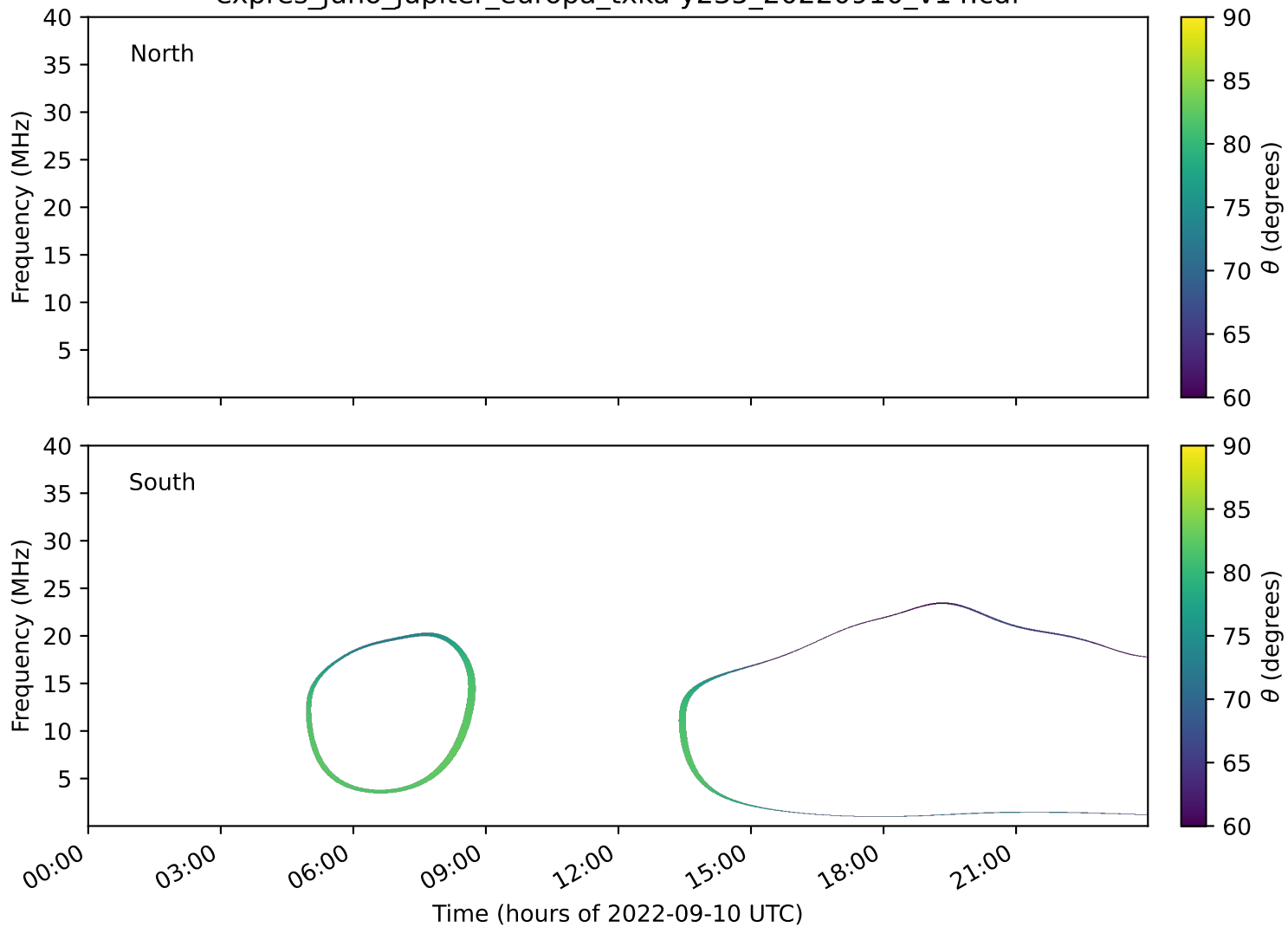
expres_juno_jupiter_europa_txka-y235_20220910_v14.cdf
