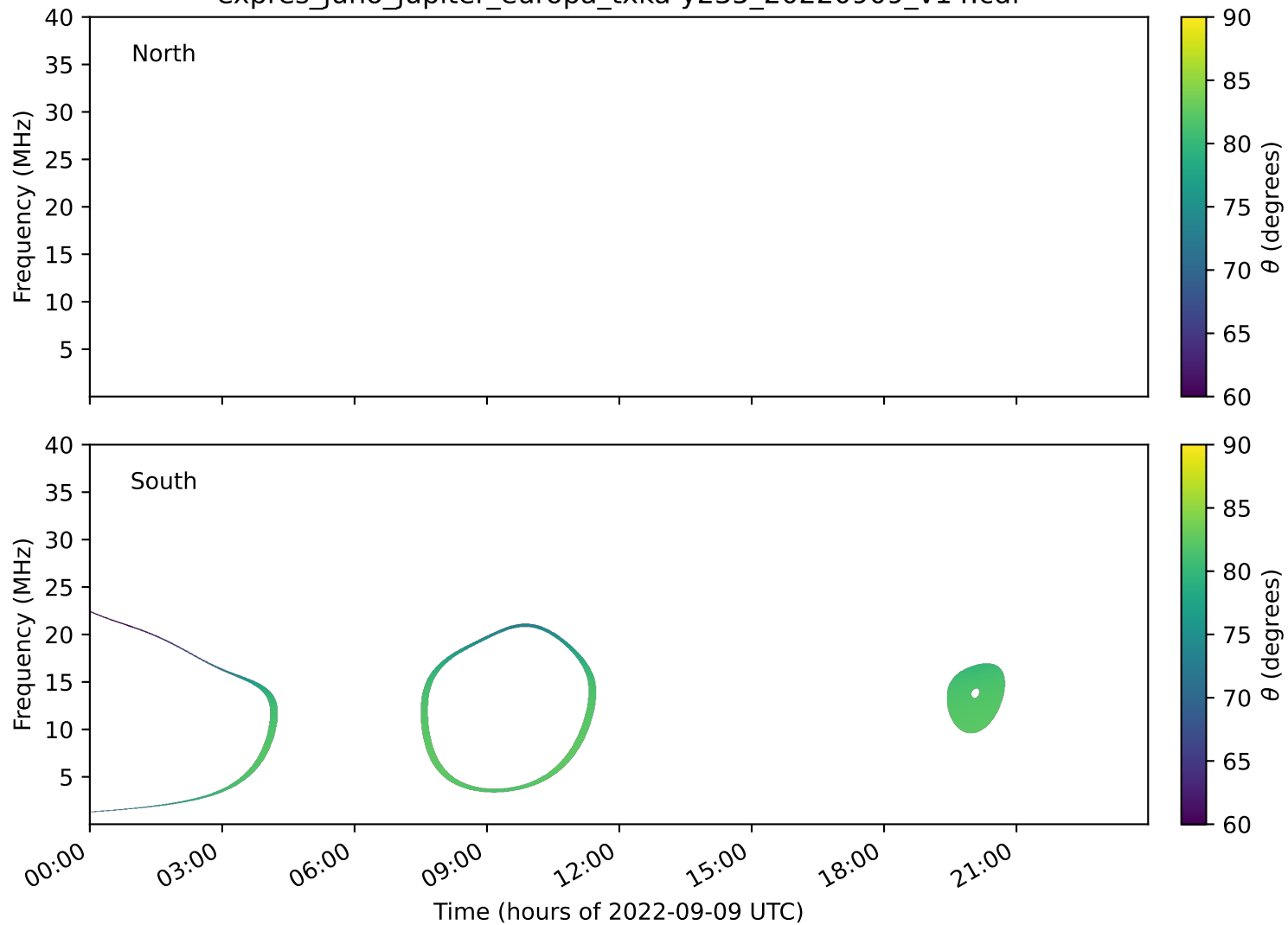
expres_juno_jupiter_europa_txka-y235_20220909_v14.cdf
