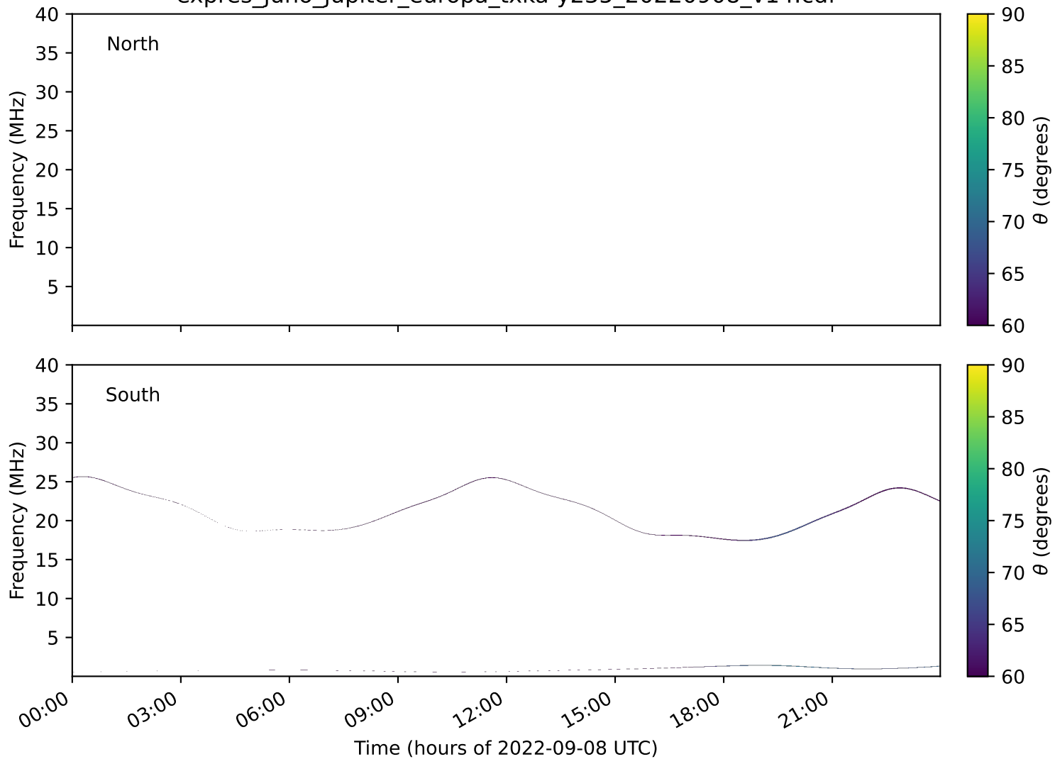
expres_juno_jupiter_europa_txka-y235_20220908_v14.cdf
