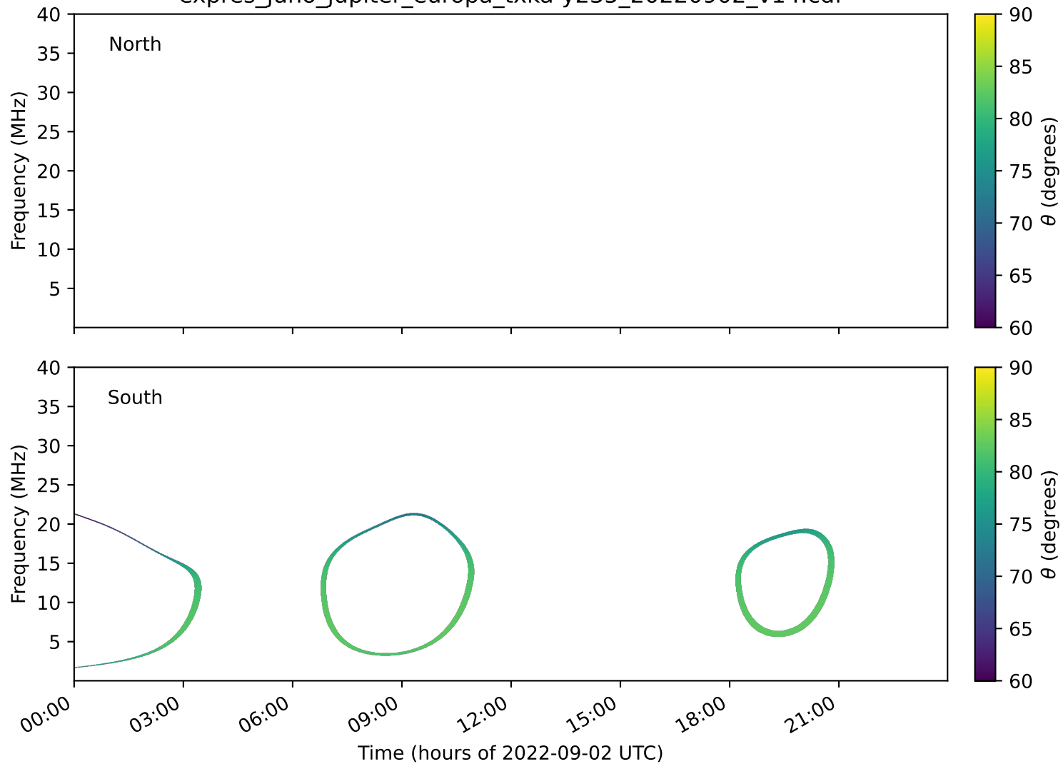
expres_juno_jupiter_europa_txka-y235_20220902_v14.cdf
