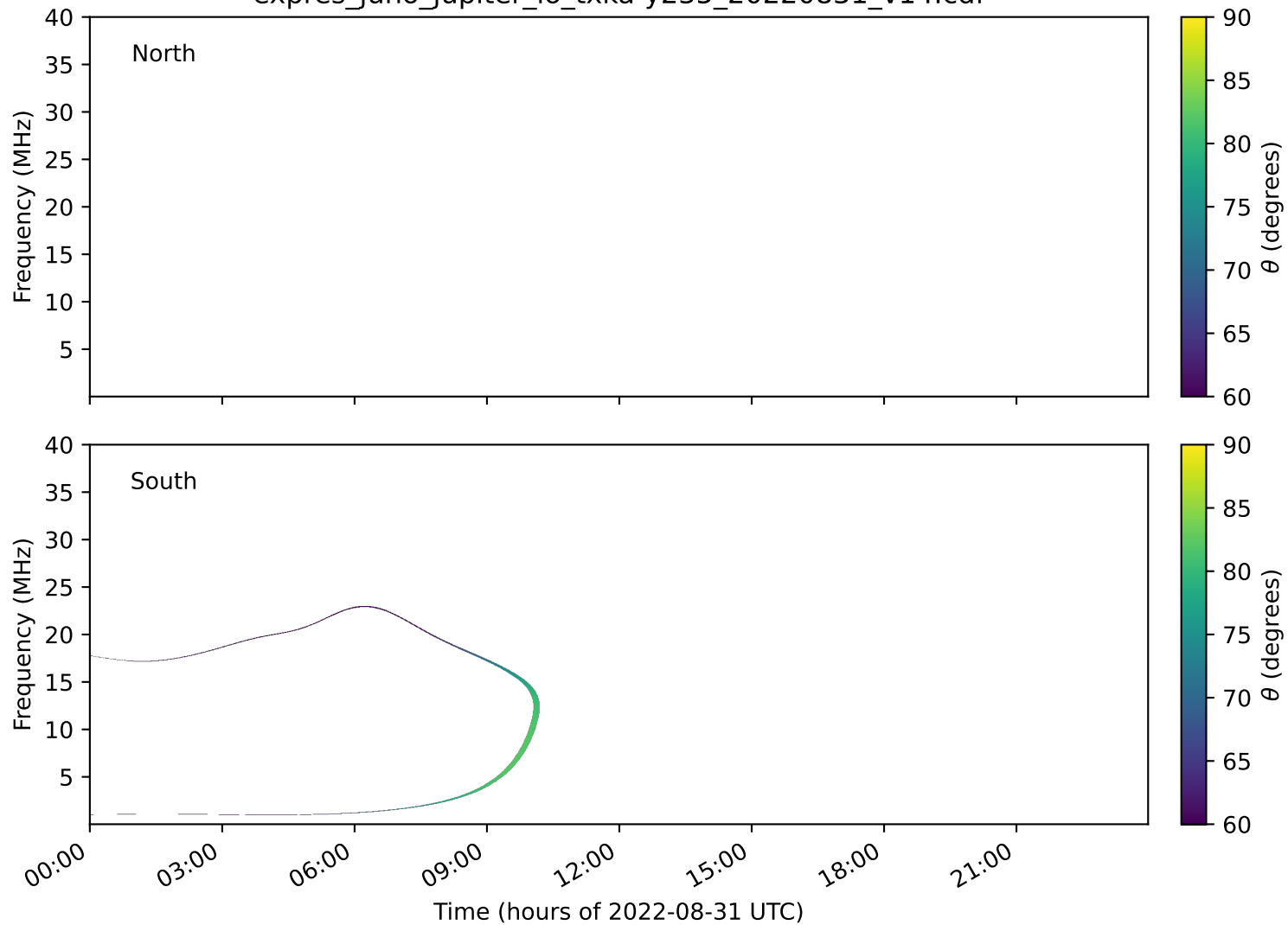
expres_juno_jupiter_io_txka-y235_20220831_v14.cdf
