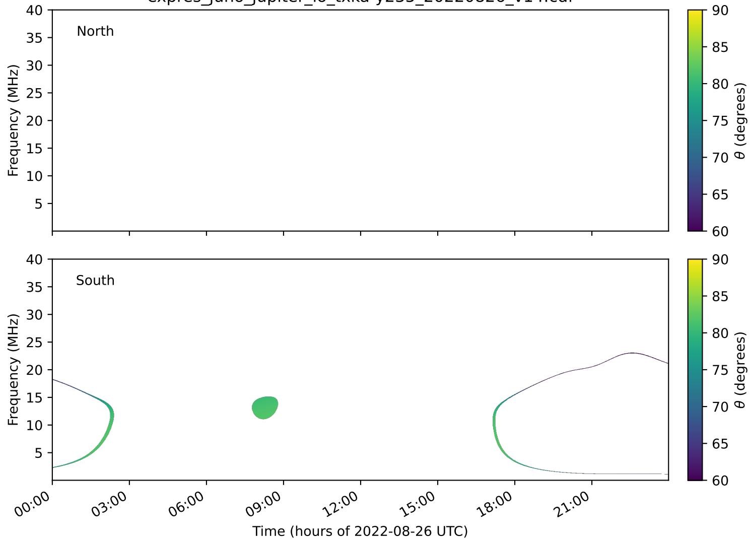
expres_juno_jupiter_io_txka-y235_20220826_v14.cdf
