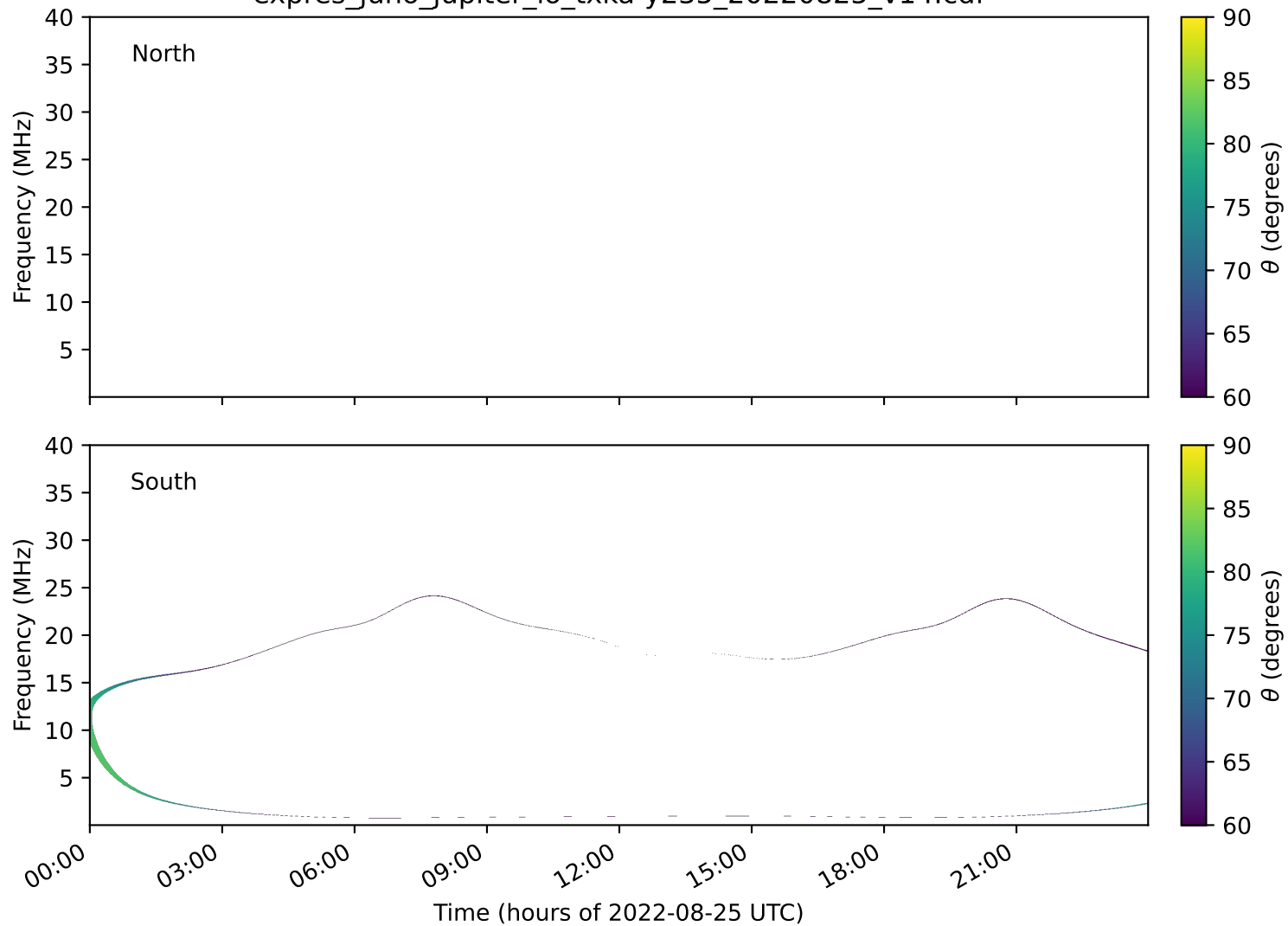
expres_juno_jupiter_io_txka-y235_20220825_v14.cdf
