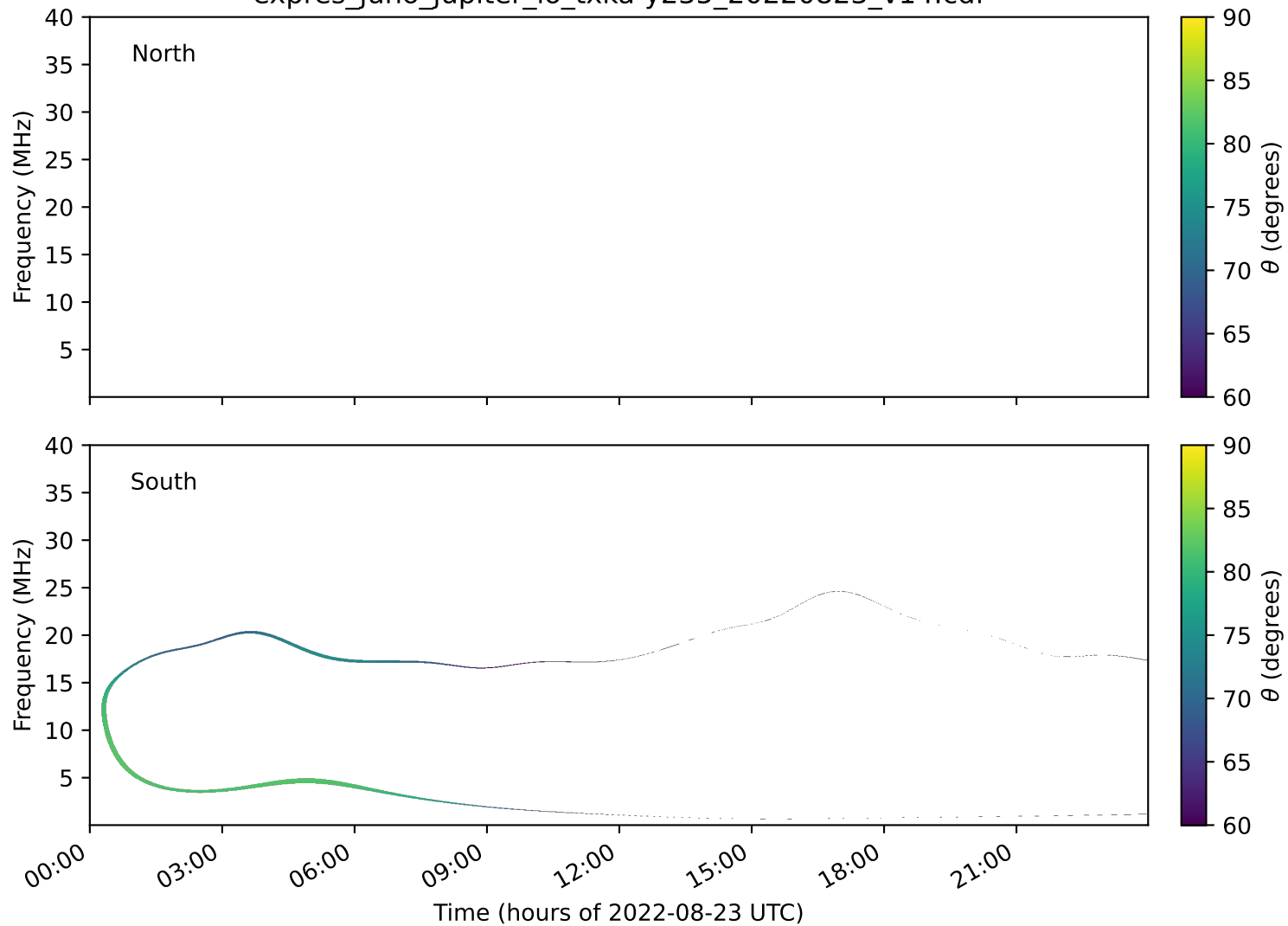
expres_juno_jupiter_io_txka-y235_20220823_v14.cdf
