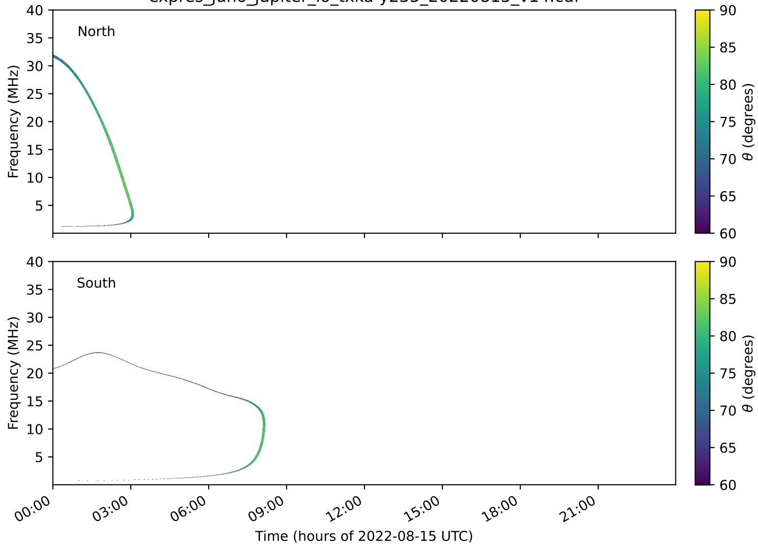
expres_juno_jupiter_io_txka-y235_20220815_v14.cdf
