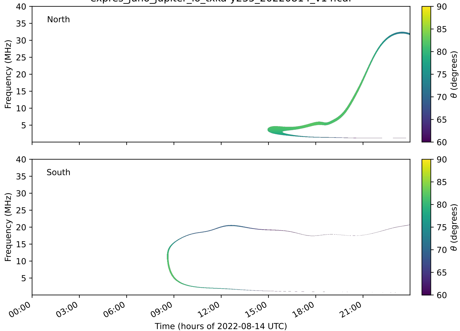
expres_juno_jupiter_io_txka-y235_20220814_v14.cdf
