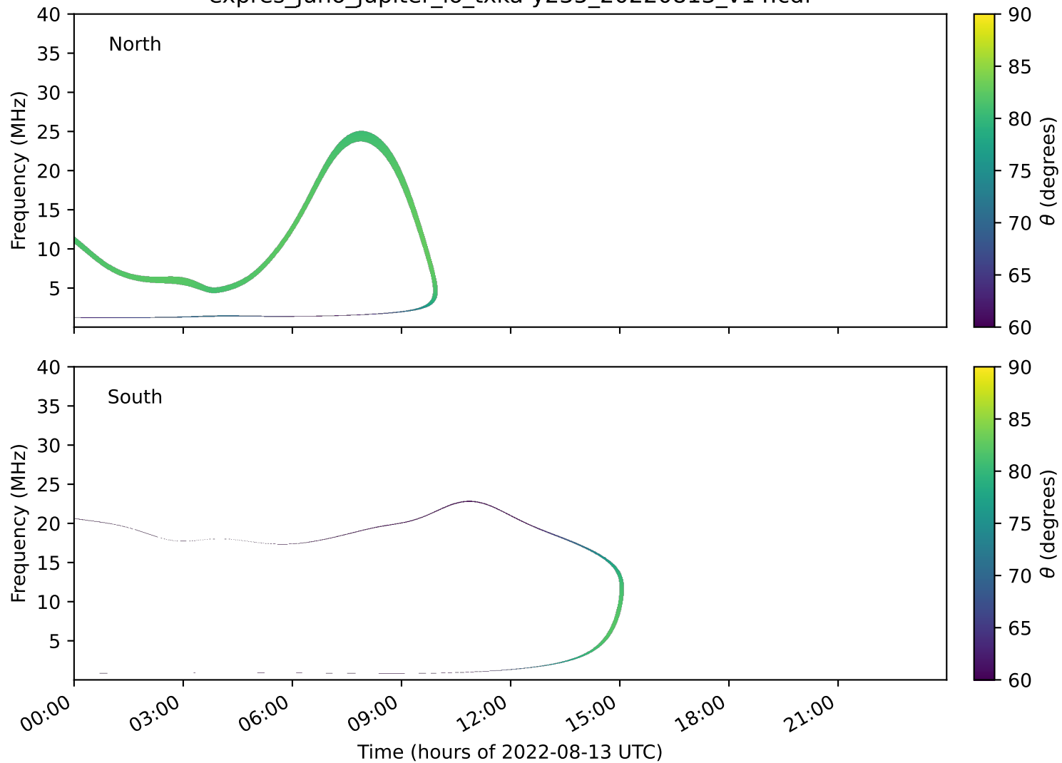
expres_juno_jupiter_io_txka-y235_20220813_v14.cdf
