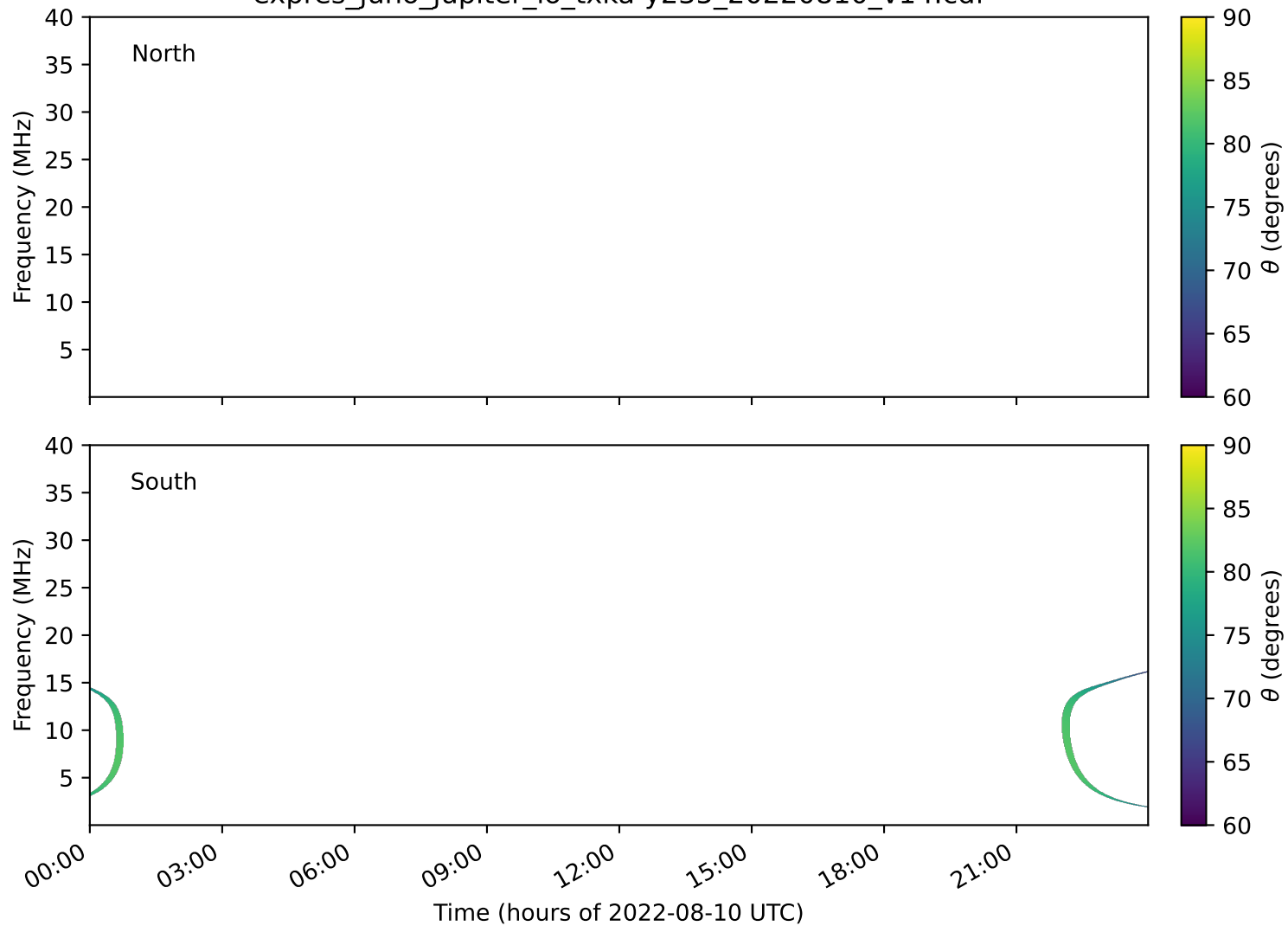
expres_juno_jupiter_io_txka-y235_20220810_v14.cdf
