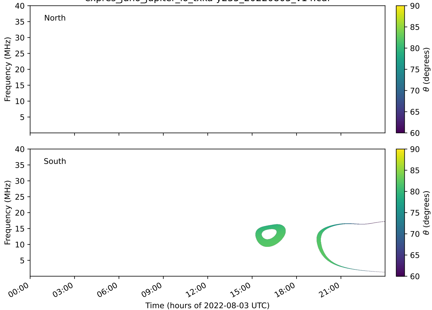
expres_juno_jupiter_io_txka-y235_20220803_v14.cdf
