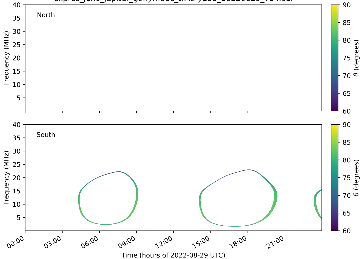
expres_juno_jupiter_ganymede_txka-y235_20220829_v14.cdf
