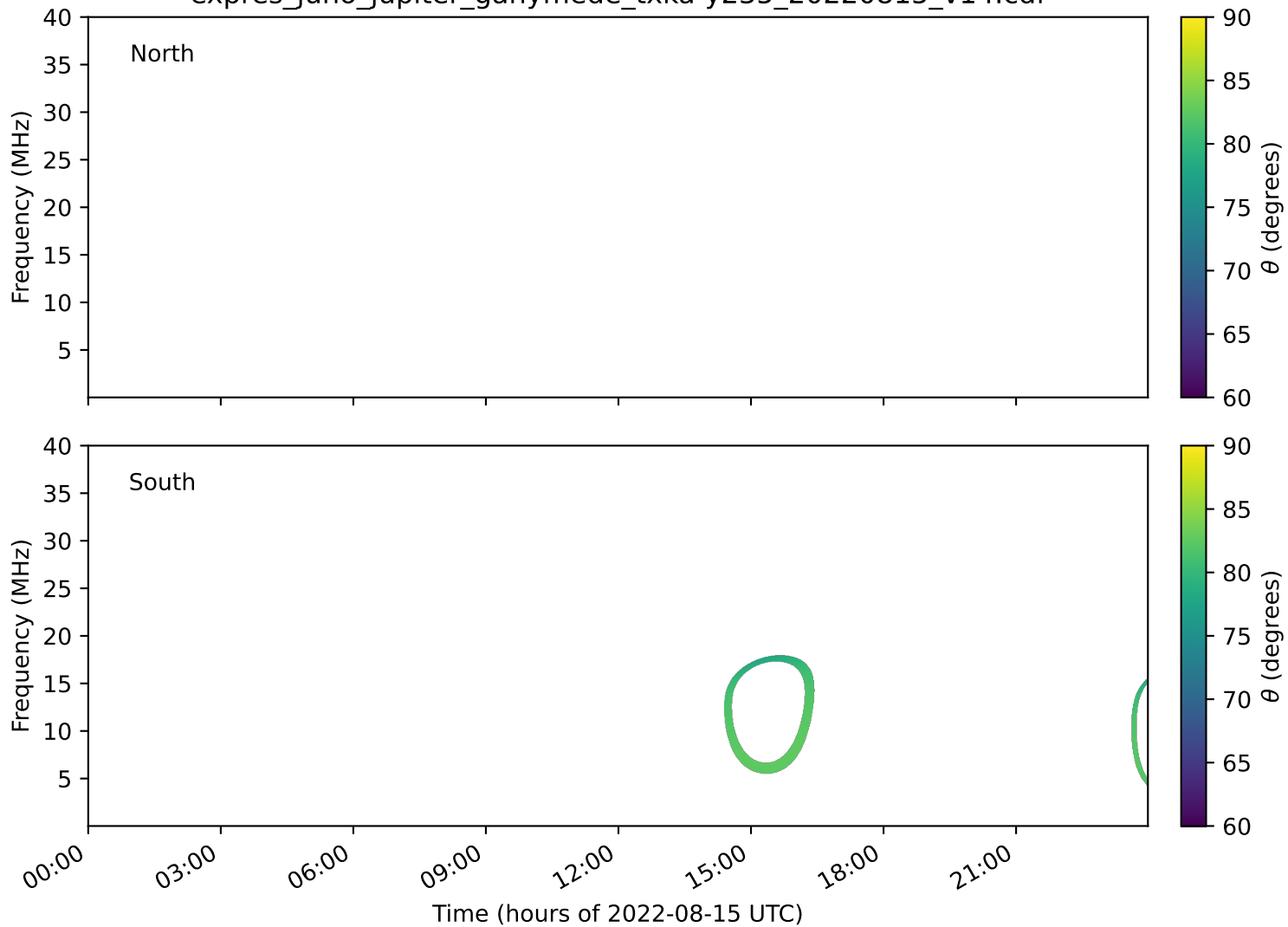
expres_juno_jupiter_ganymede_txka-y235_20220815_v14.cdf
