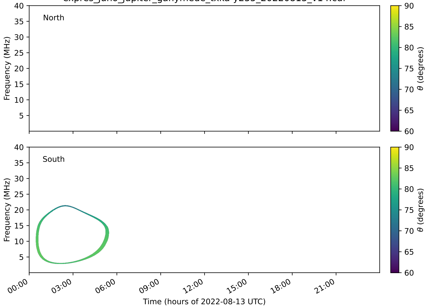
expres_juno_jupiter_ganymede_txka-y235_20220813_v14.cdf
