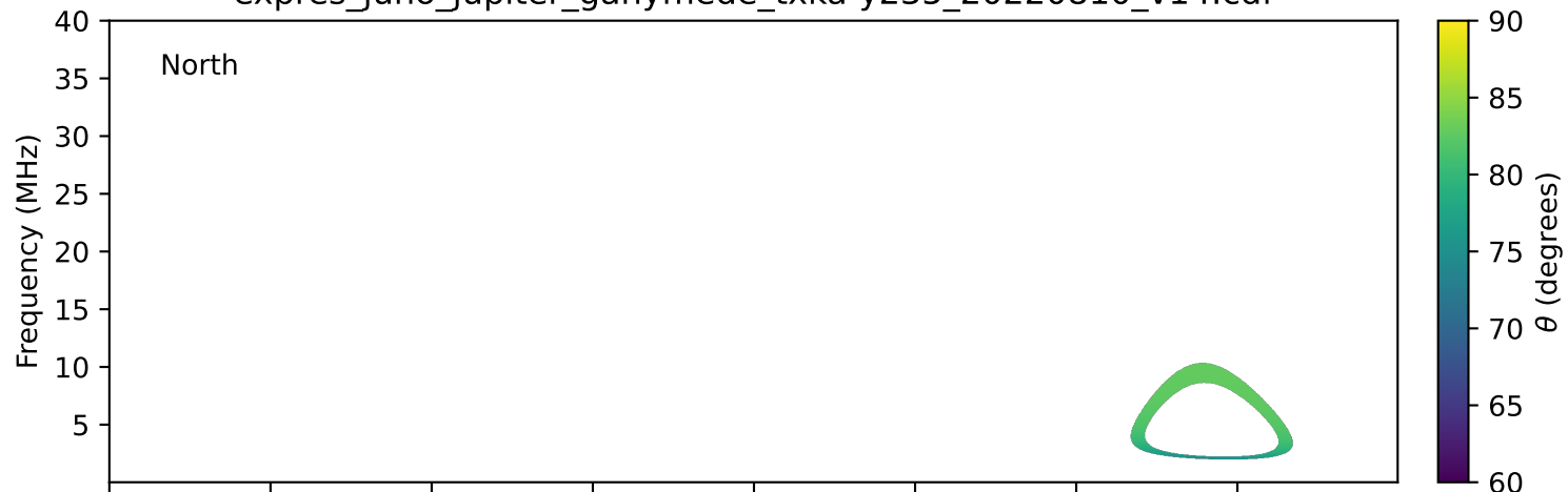
expres_juno_jupiter_ganymede_txka-y235_20220810_v14.cdf
