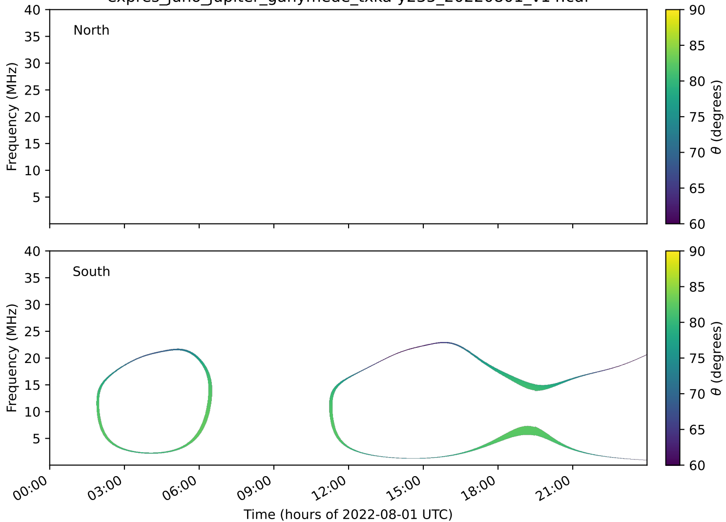
expres_juno_jupiter_ganymede_txka-y235_20220801_v14.cdf
