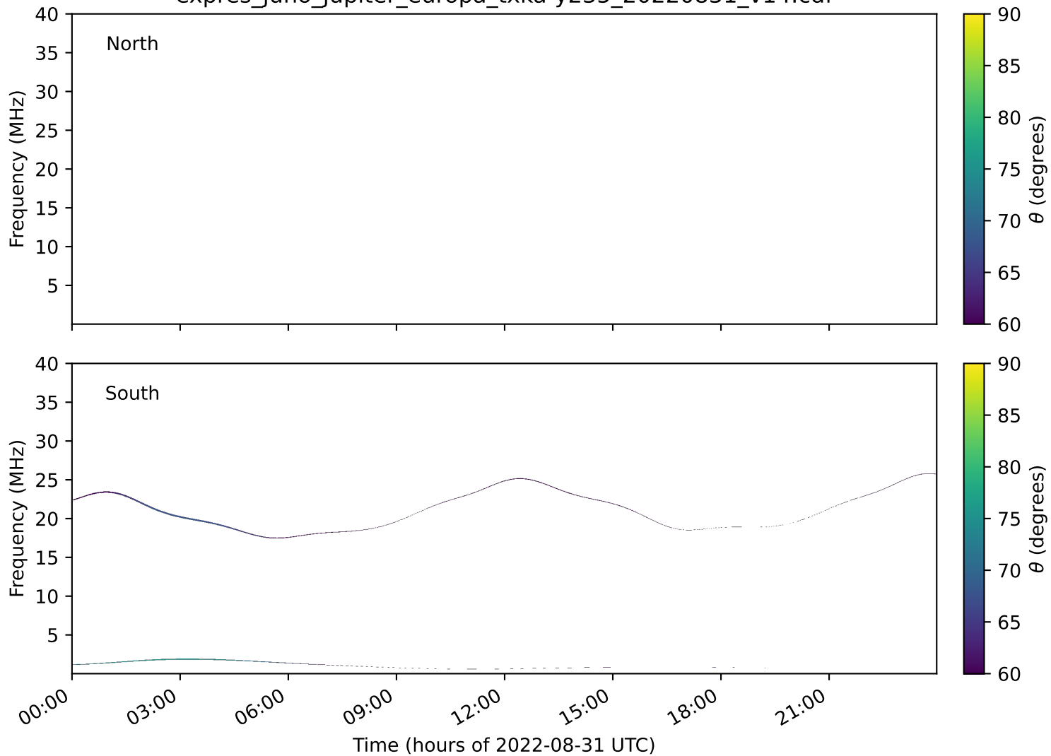
expres_juno_jupiter_europa_txka-y235_20220831_v14.cdf
