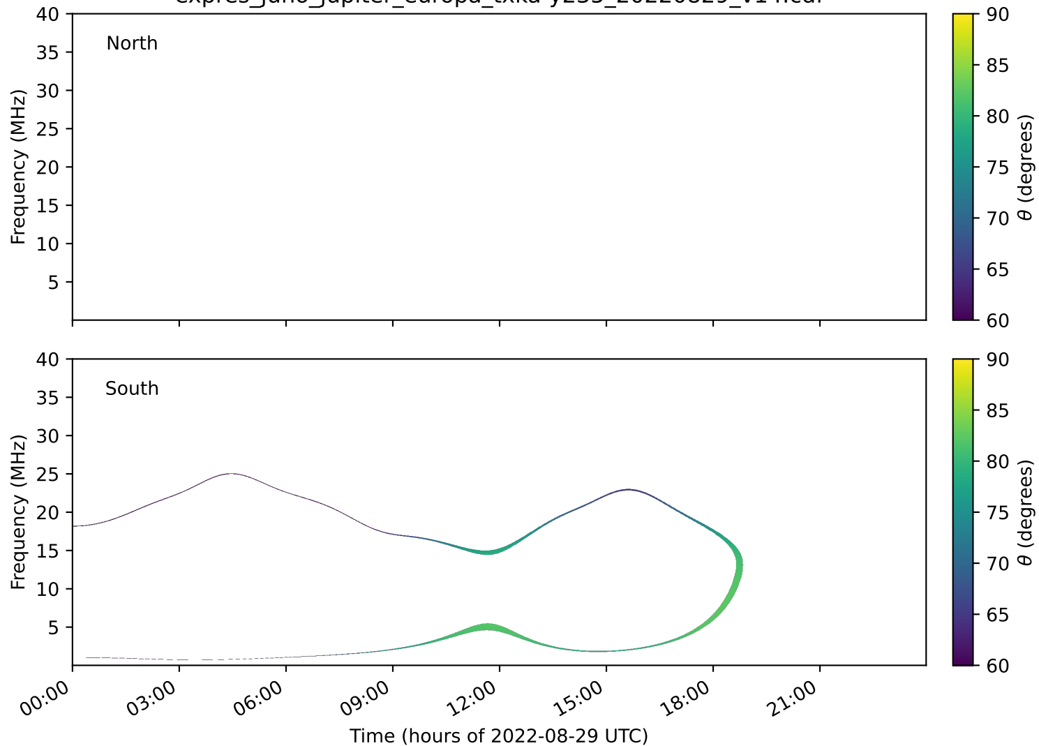
expres_juno_jupiter_europa_txka-y235_20220829_v14.cdf
