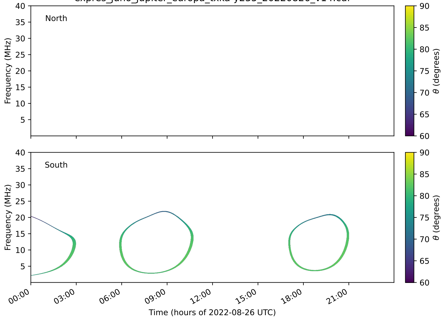
expres_juno_jupiter_europa_txka-y235_20220826_v14.cdf
