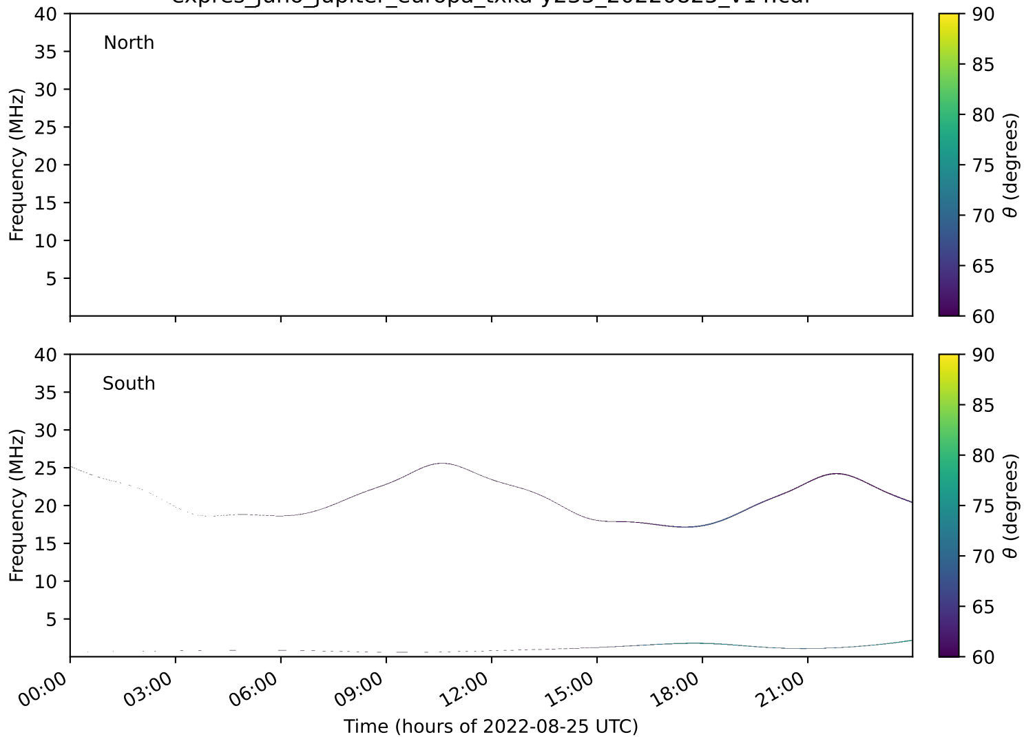
expres_juno_jupiter_europa_txka-y235_20220825_v14.cdf
