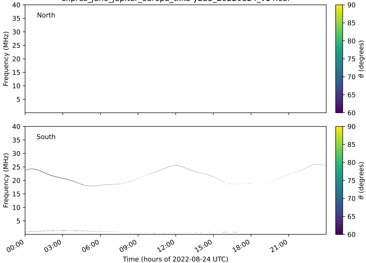
expres_juno_jupiter_europa_txka-y235_20220824_v14.cdf
