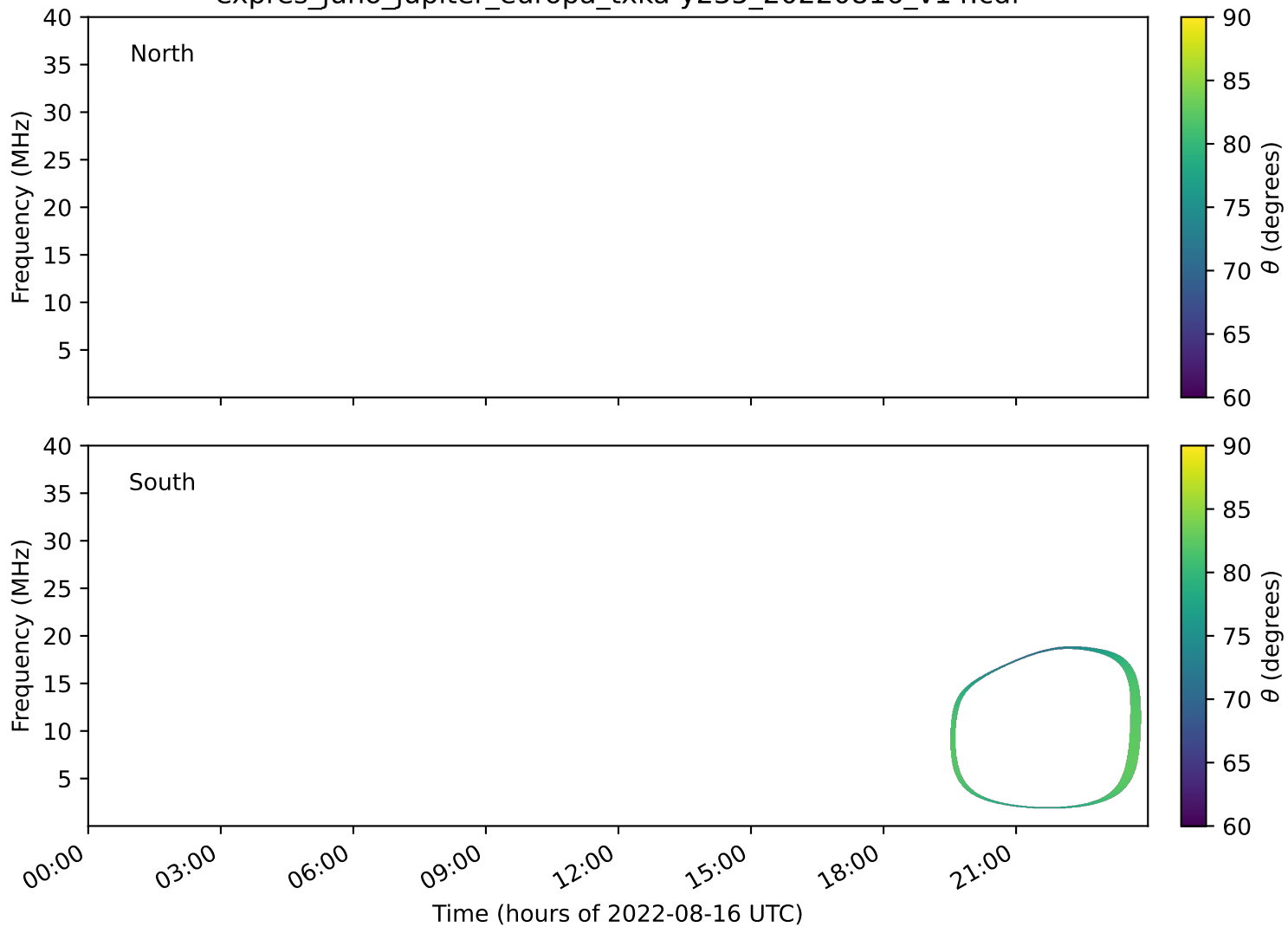
expres_juno_jupiter_europa_txka-y235_20220816_v14.cdf
