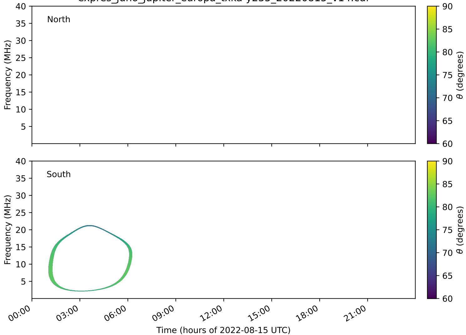
expres_juno_jupiter_europa_txka-y235_20220815_v14.cdf
