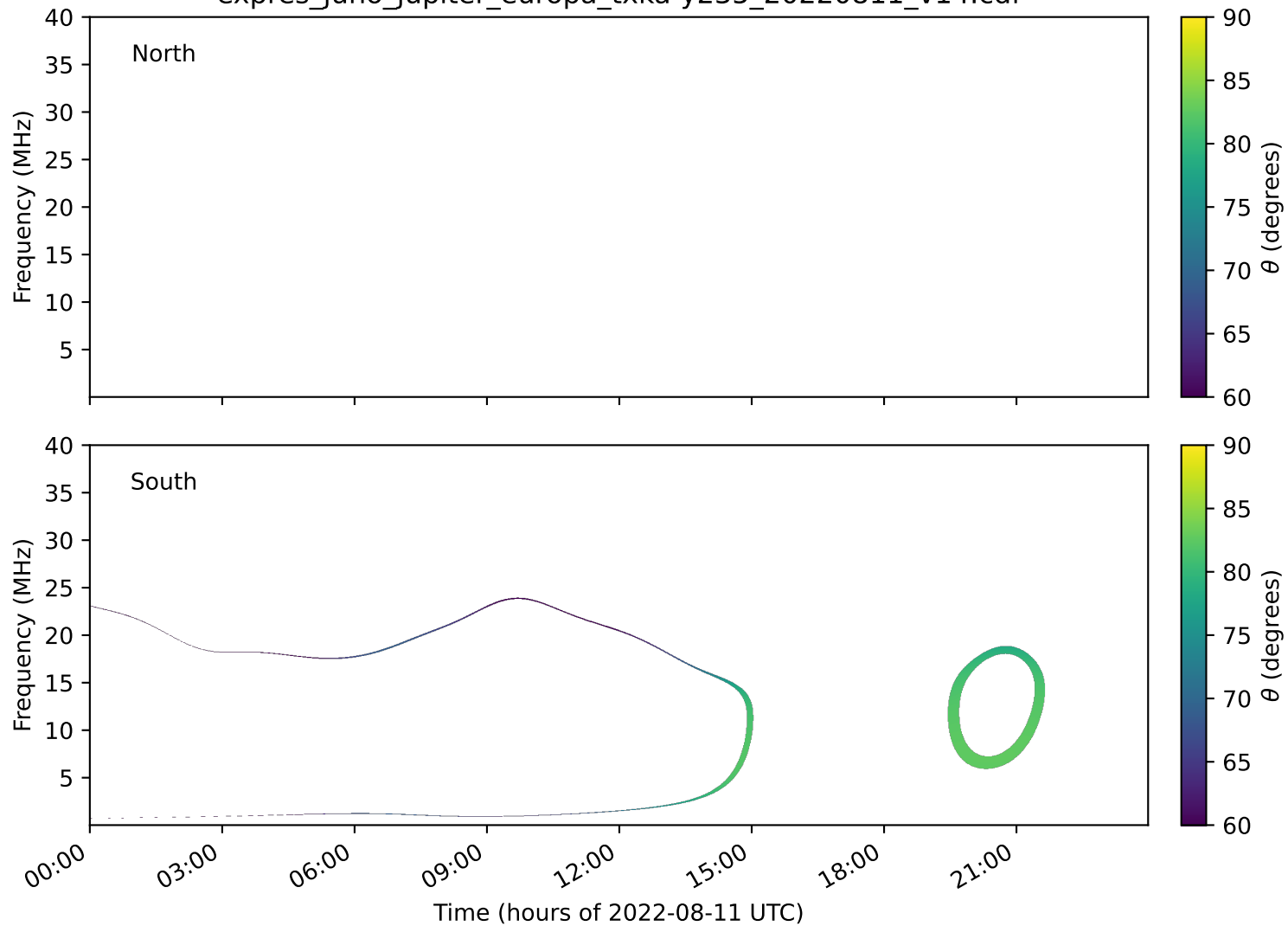
expres_juno_jupiter_europa_txka-y235_20220811_v14.cdf
