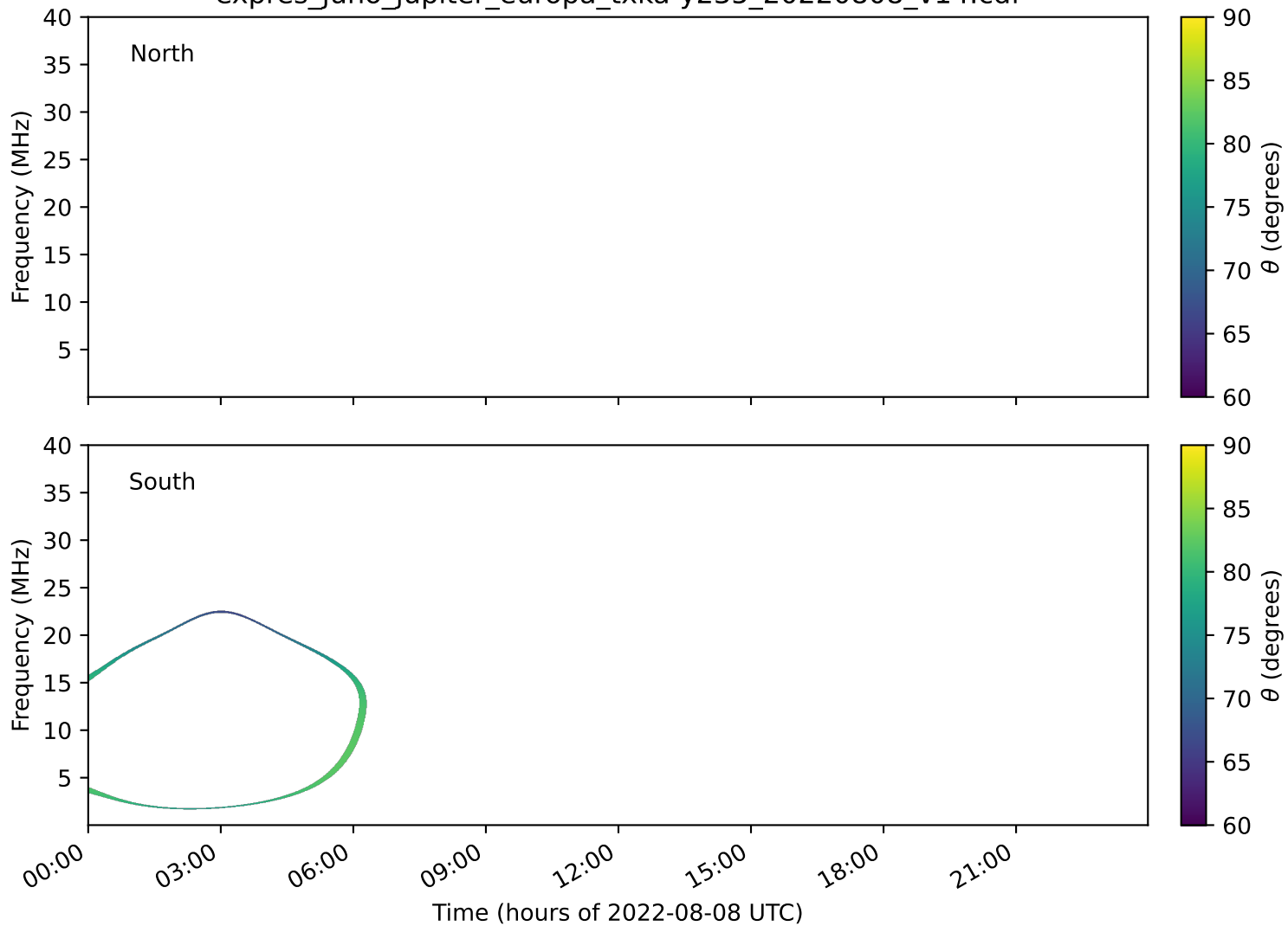
expres_juno_jupiter_europa_txka-y235_20220808_v14.cdf
