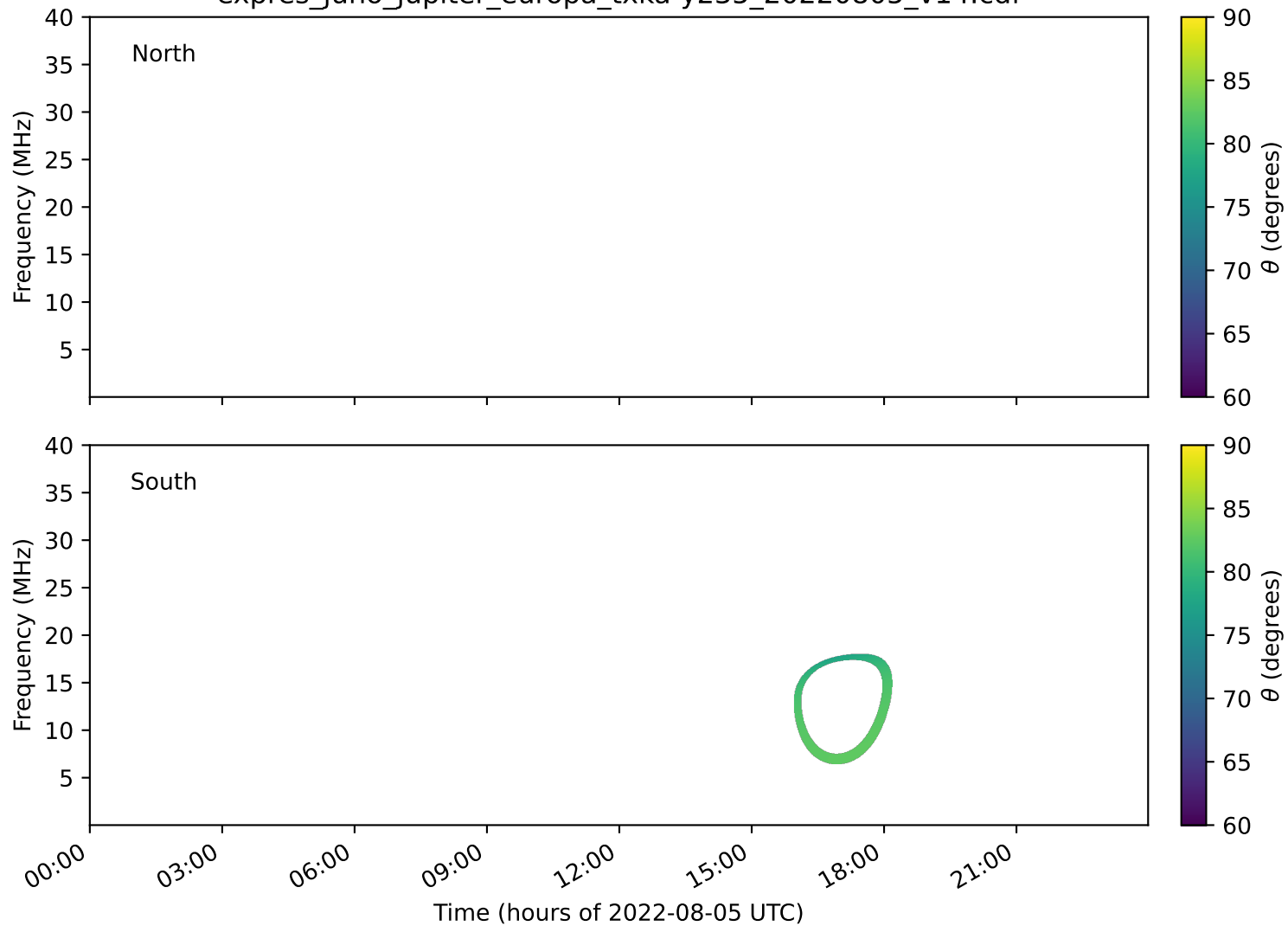
expres_juno_jupiter_europa_txka-y235_20220805_v14.cdf
