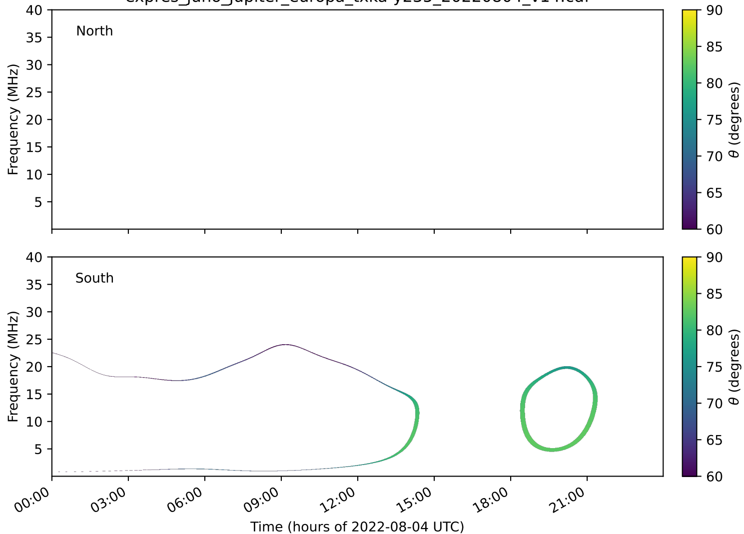
expres_juno_jupiter_europa_txka-y235_20220804_v14.cdf
