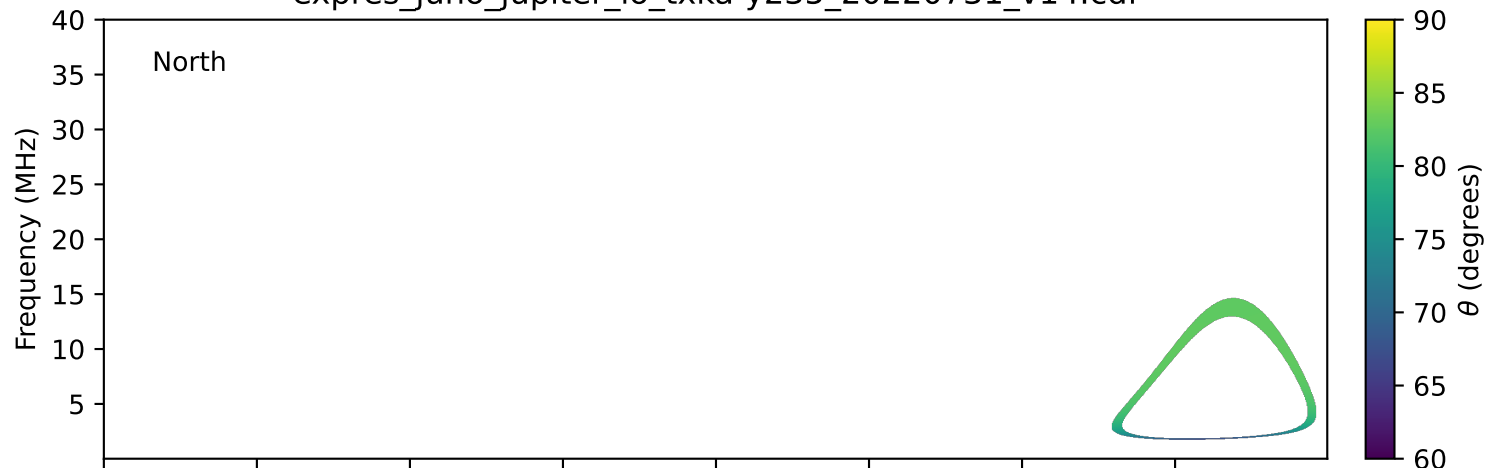
expres_juno_jupiter_io_txka-y235_20220731_v14.cdf
