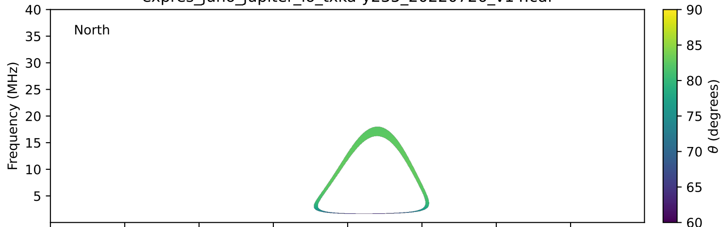
expres_juno_jupiter_io_txka-y235_20220726_v14.cdf
