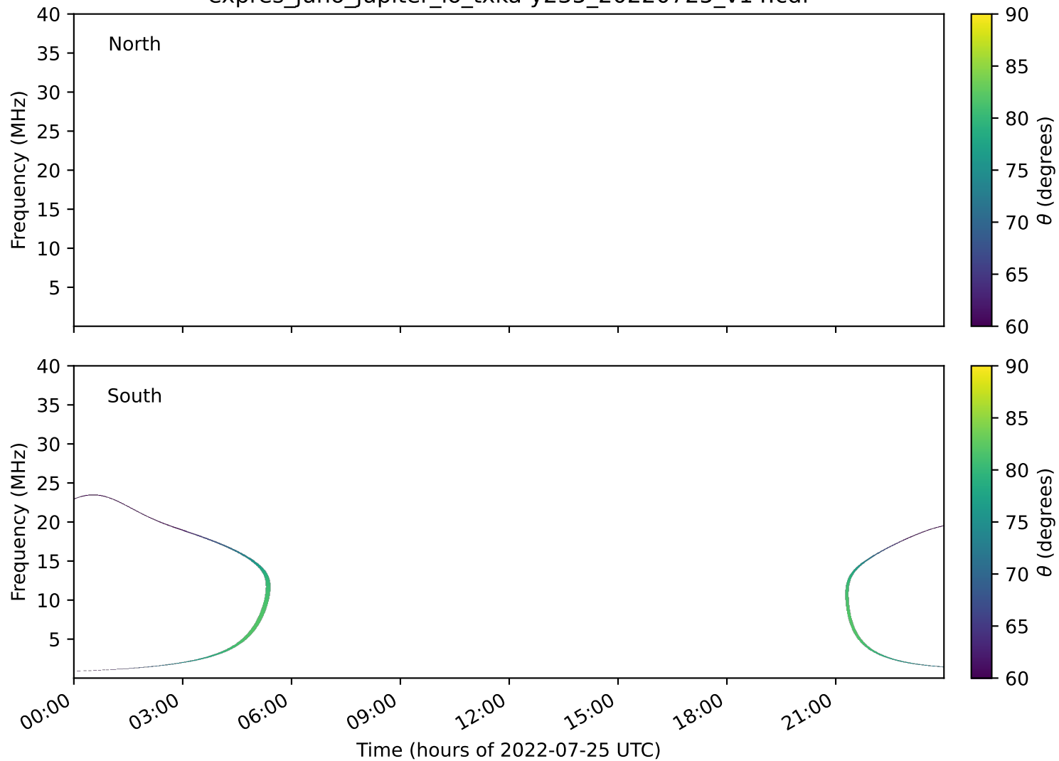
expres_juno_jupiter_io_txka-y235_20220725_v14.cdf
