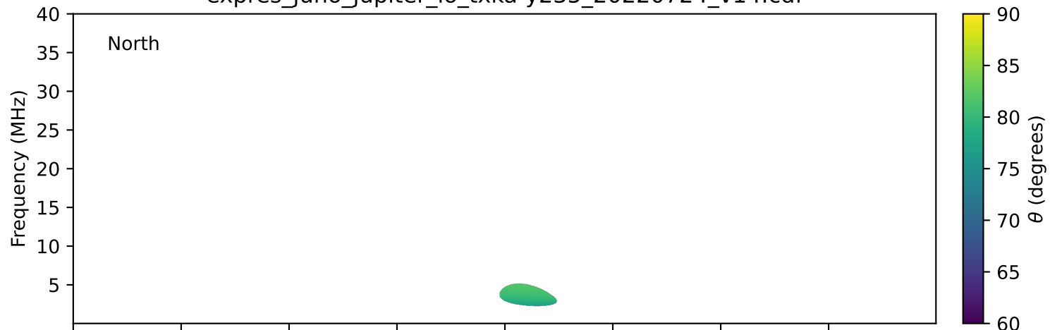
expres_juno_jupiter_io_txka-y235_20220724_v14.cdf
