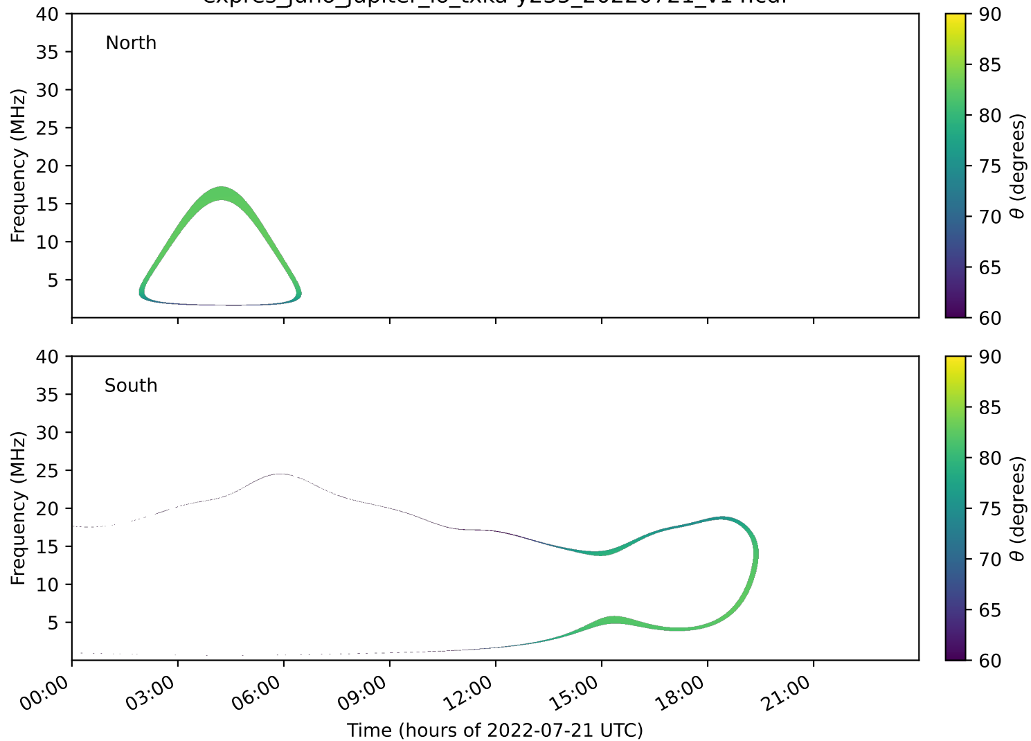
expres_juno_jupiter_io_txka-y235_20220721_v14.cdf
