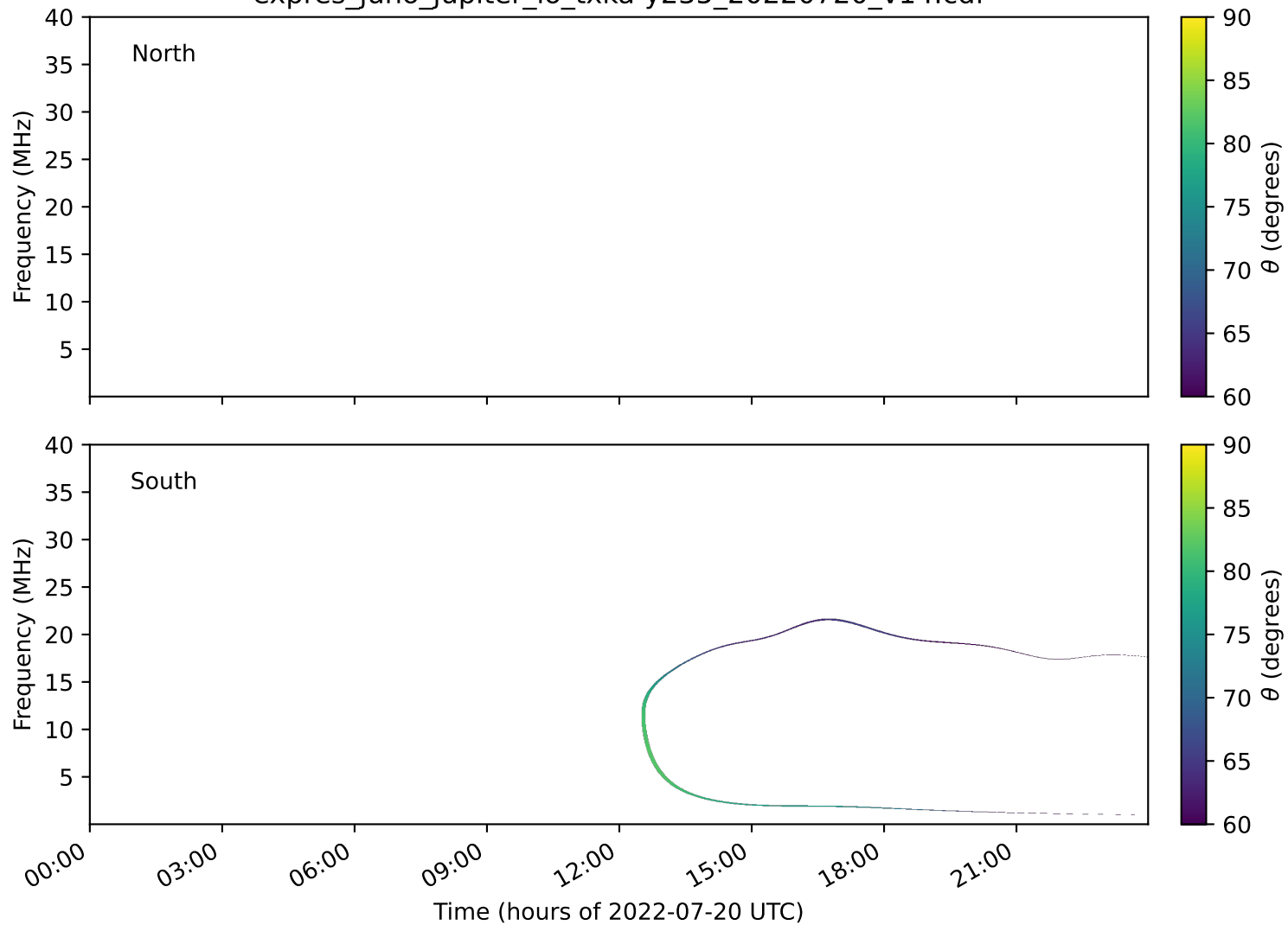
expres_juno_jupiter_io_txka-y235_20220720_v14.cdf
