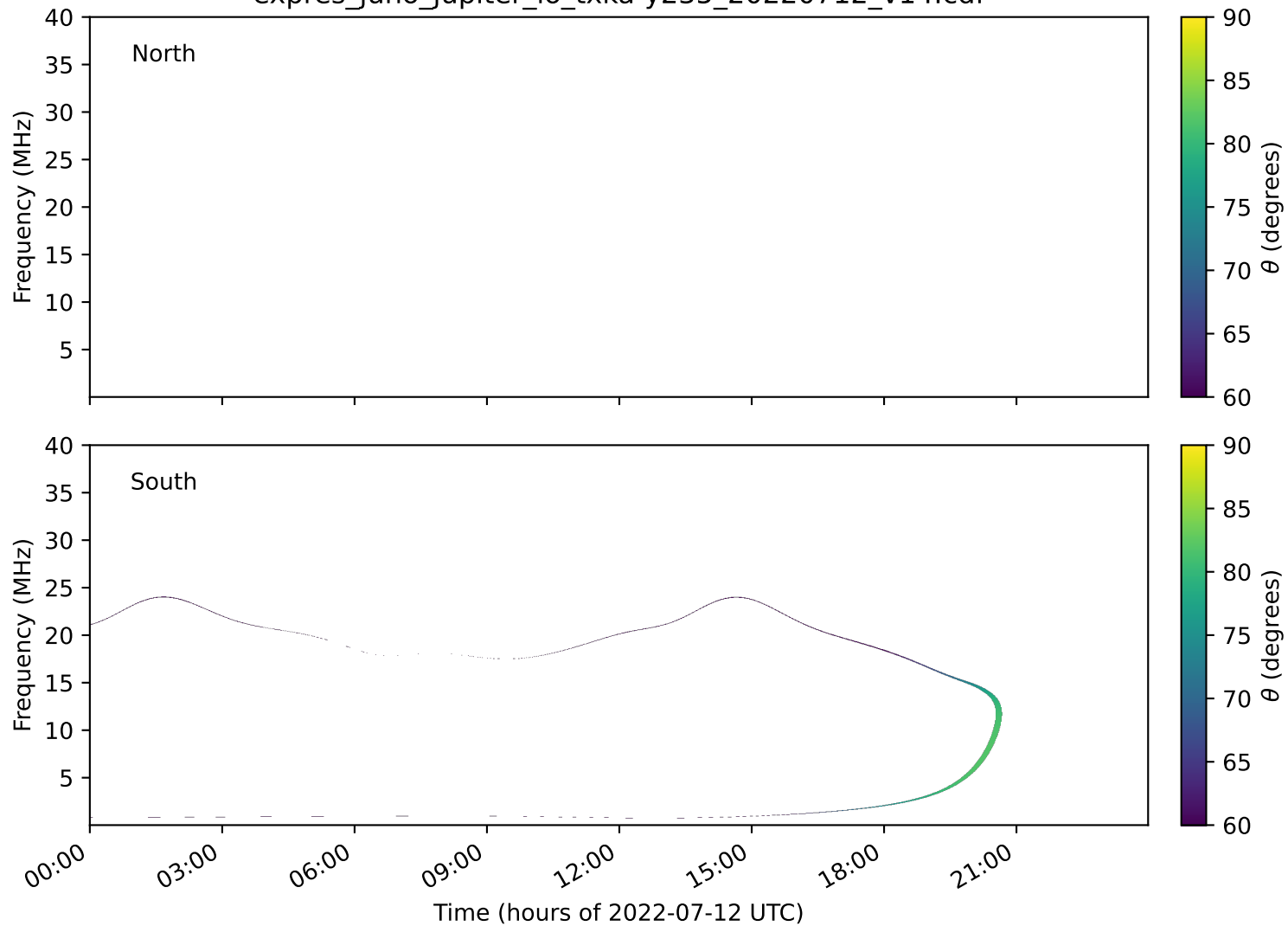
expres_juno_jupiter_io_txka-y235_20220712_v14.cdf
