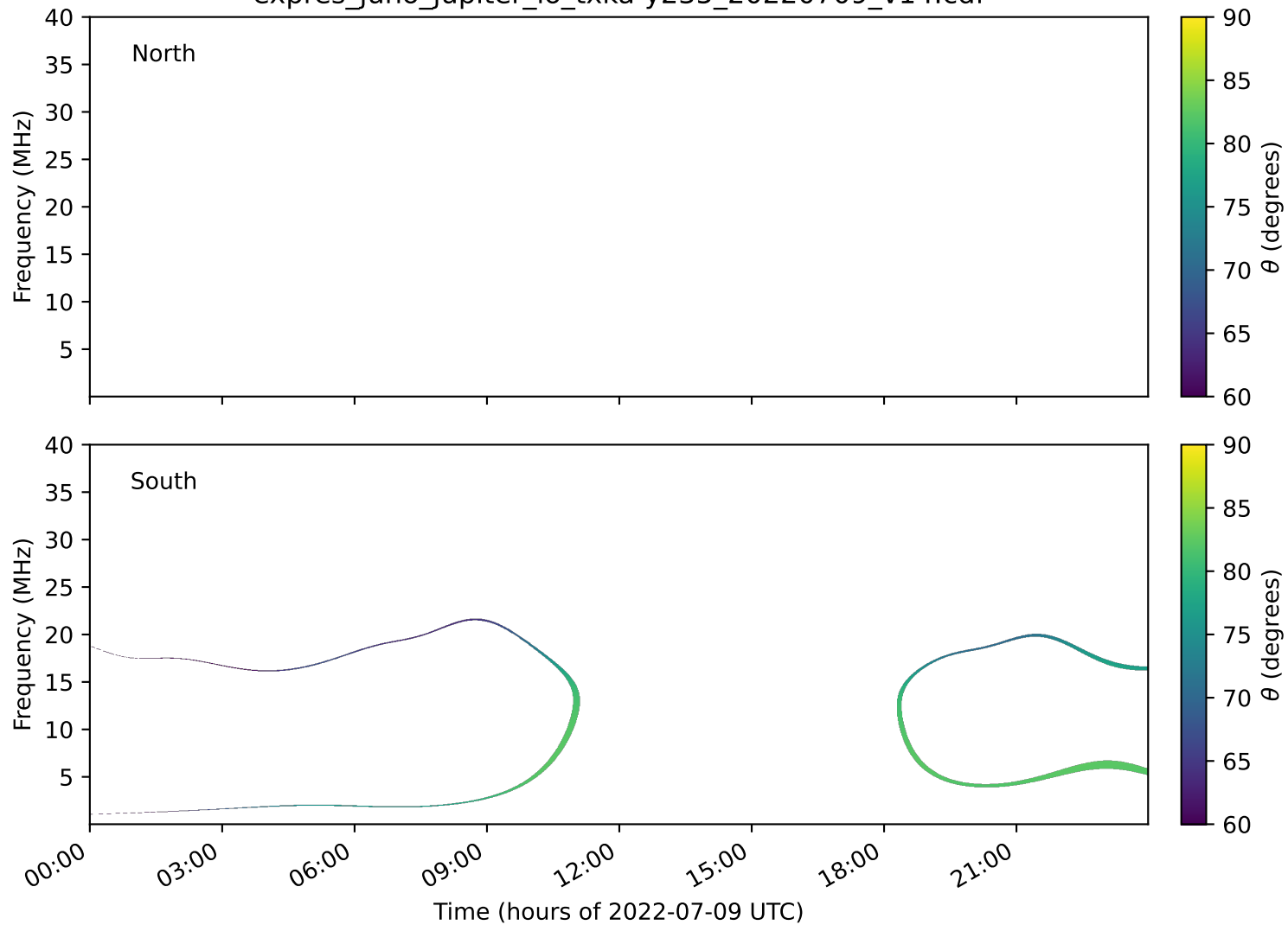
expres_juno_jupiter_io_txka-y235_20220709_v14.cdf
