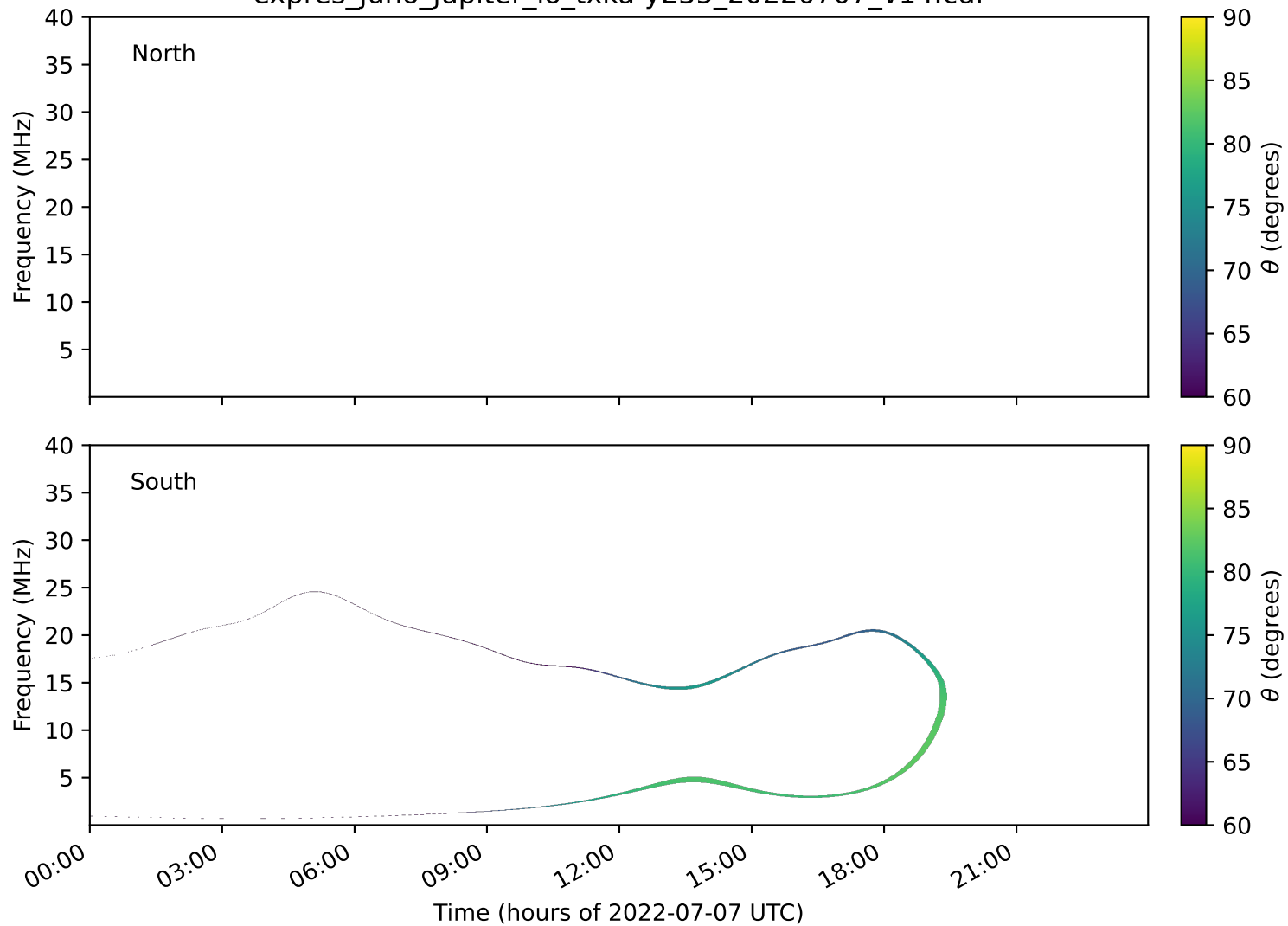
expres_juno_jupiter_io_txka-y235_20220707_v14.cdf
