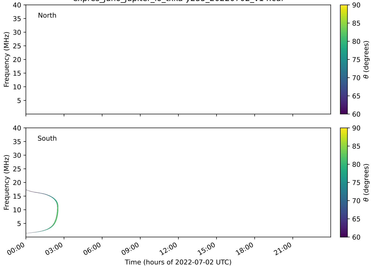
expres_juno_jupiter_io_txka-y235_20220702_v14.cdf
