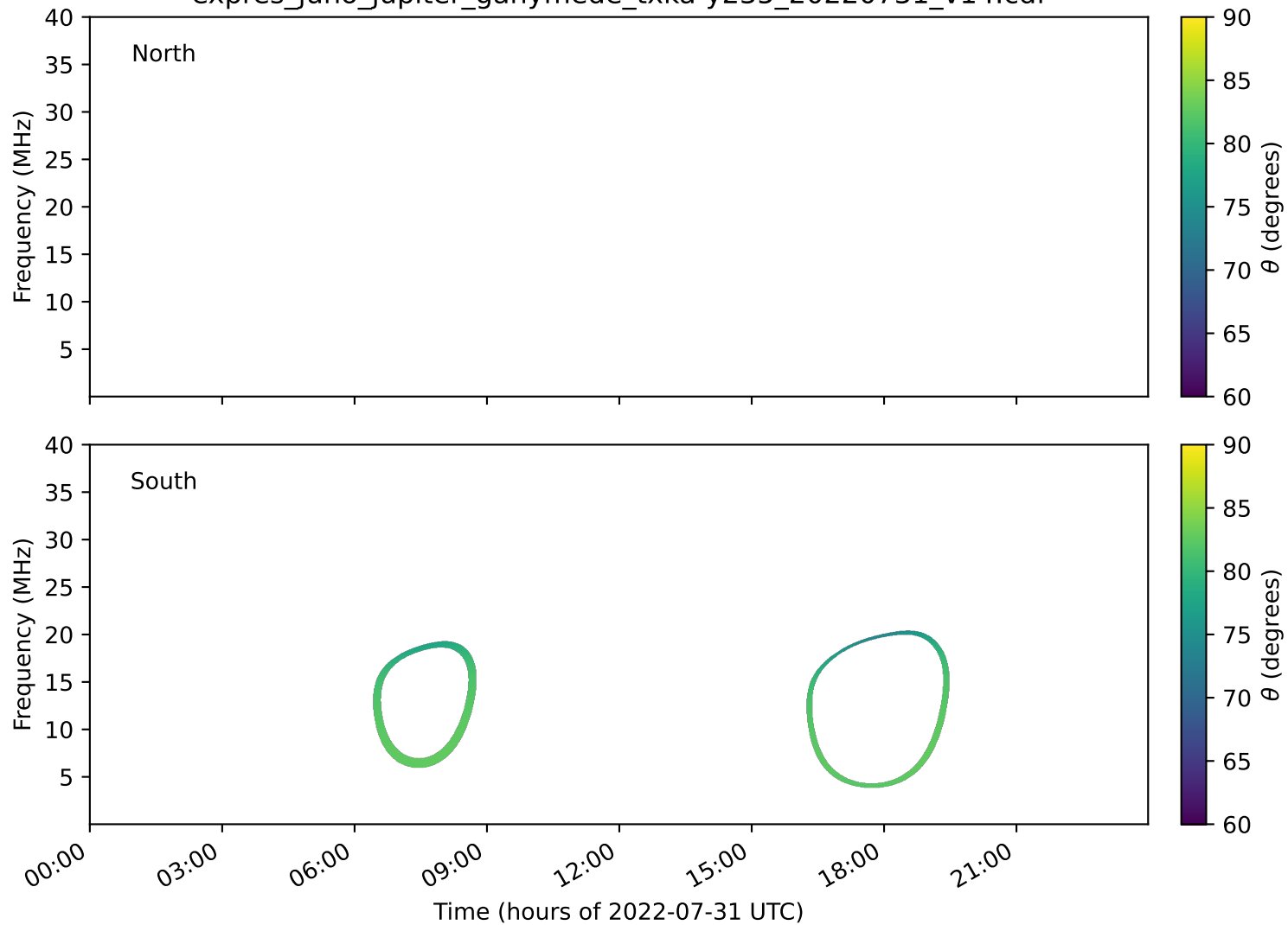
expres_juno_jupiter_ganymede_txka-y235_20220731_v14.cdf
