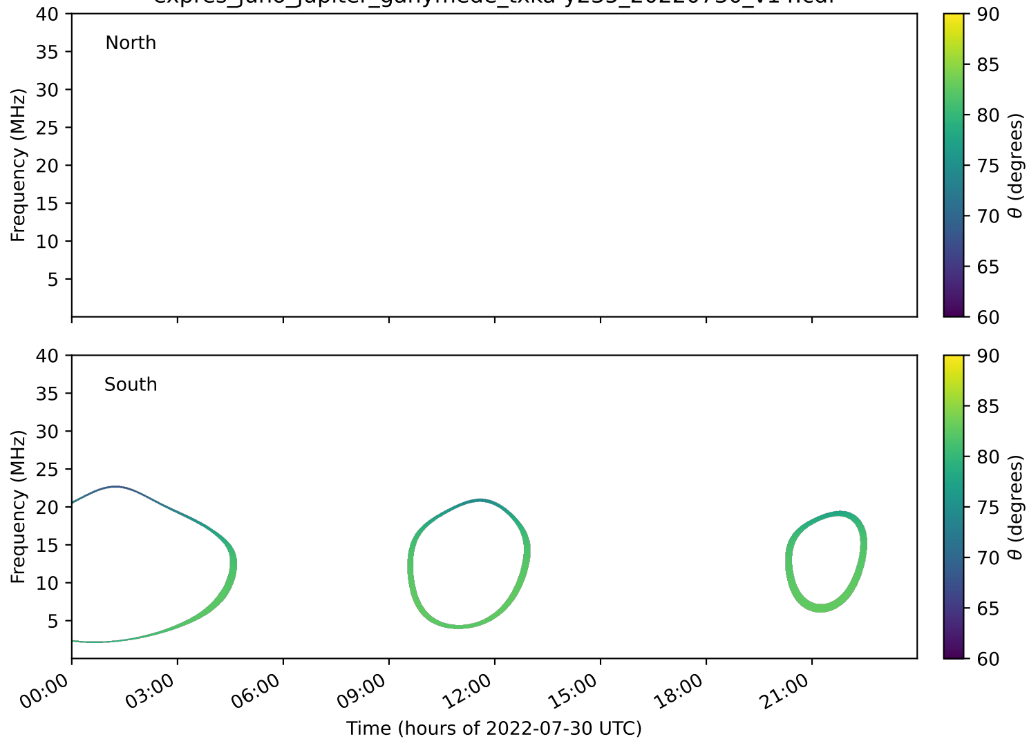
expres_juno_jupiter_ganymede_txka-y235_20220730_v14.cdf
