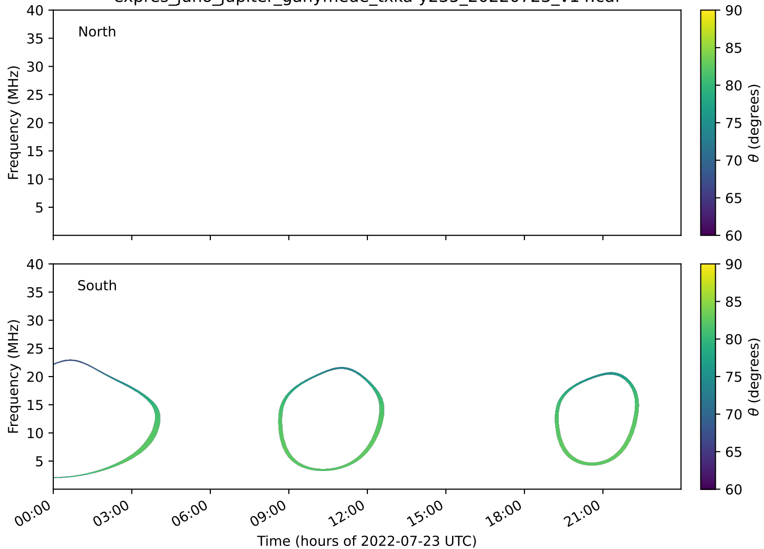
expres_juno_jupiter_ganymede_txka-y235_20220723_v14.cdf
