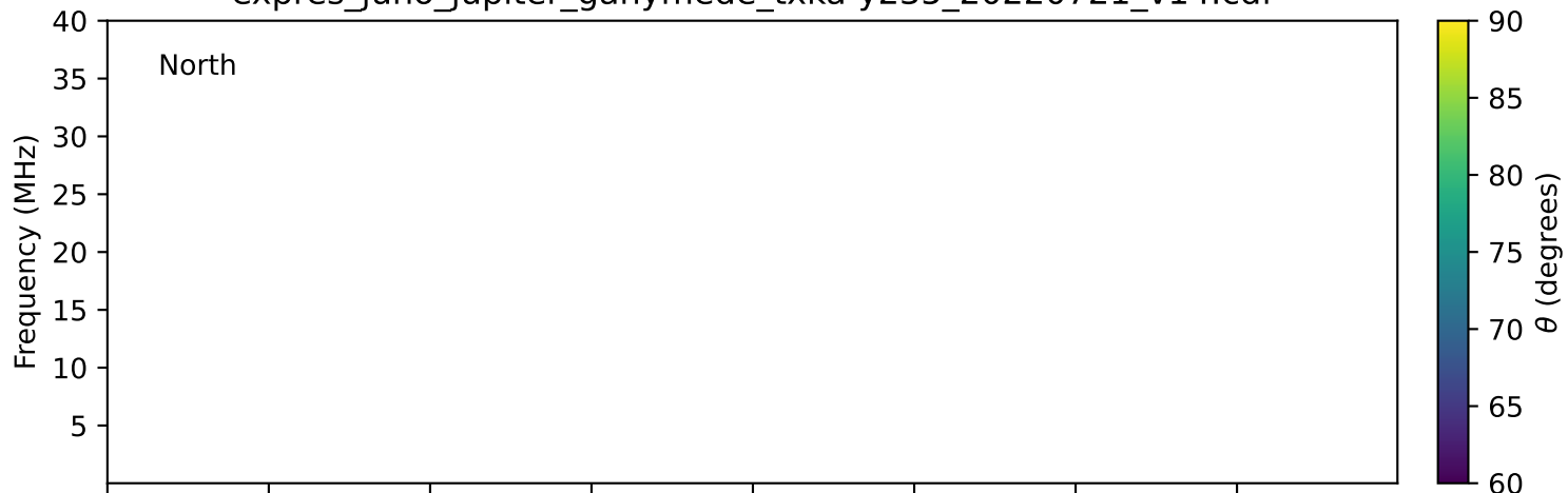
expres_juno_jupiter_ganymede_txka-y235_20220721_v14.cdf
