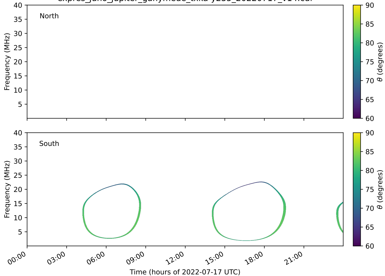
expres_juno_jupiter_ganymede_txka-y235_20220717_v14.cdf
